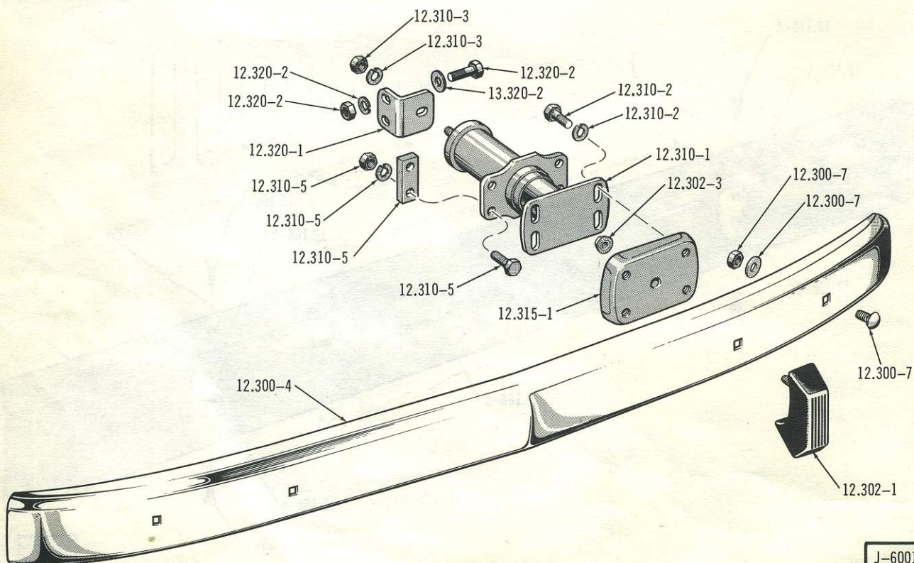
REAR BUMPER . . . 1974 80 (WEAB)
