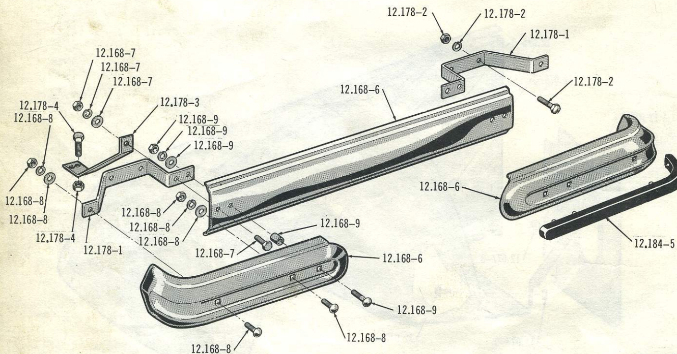
FRONT BUMPER . . . 1974/1978 10-20-40 (LEAB)
