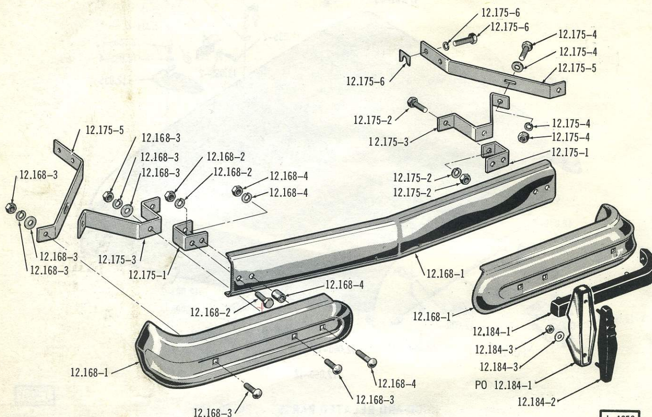
FRONT BUMPER . . . 1974/1978 10-20-40 (LEAB)
