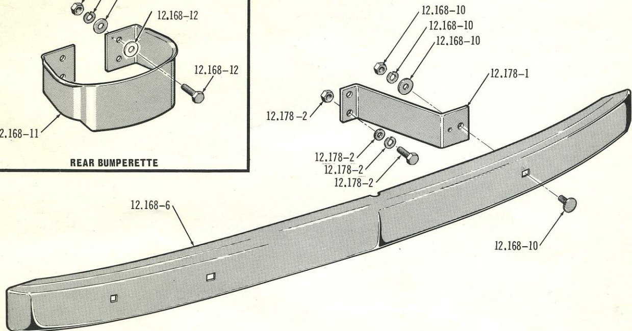
REAR BUMPER . . . 80-90 (LEAB)
