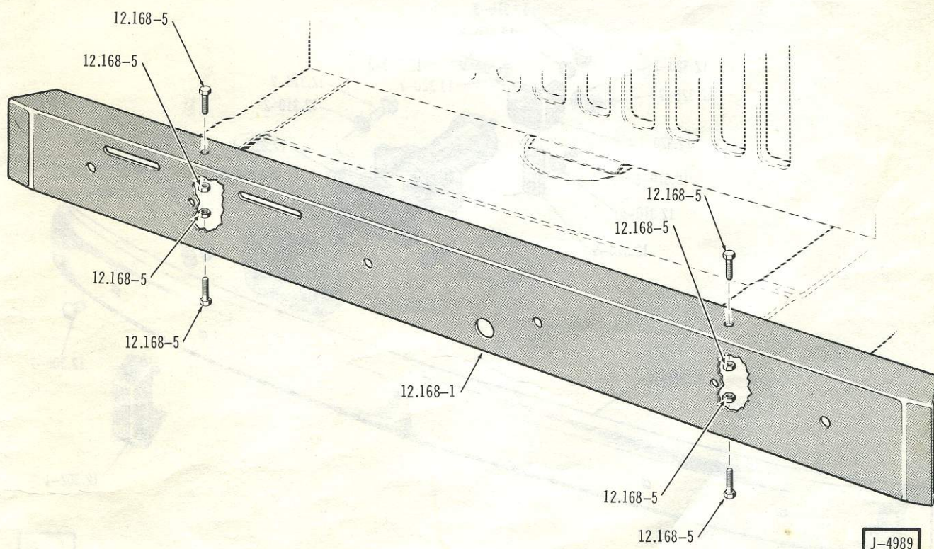
FRONT BUMPER (PAINTED) . . . 80-90 (LEAB)
