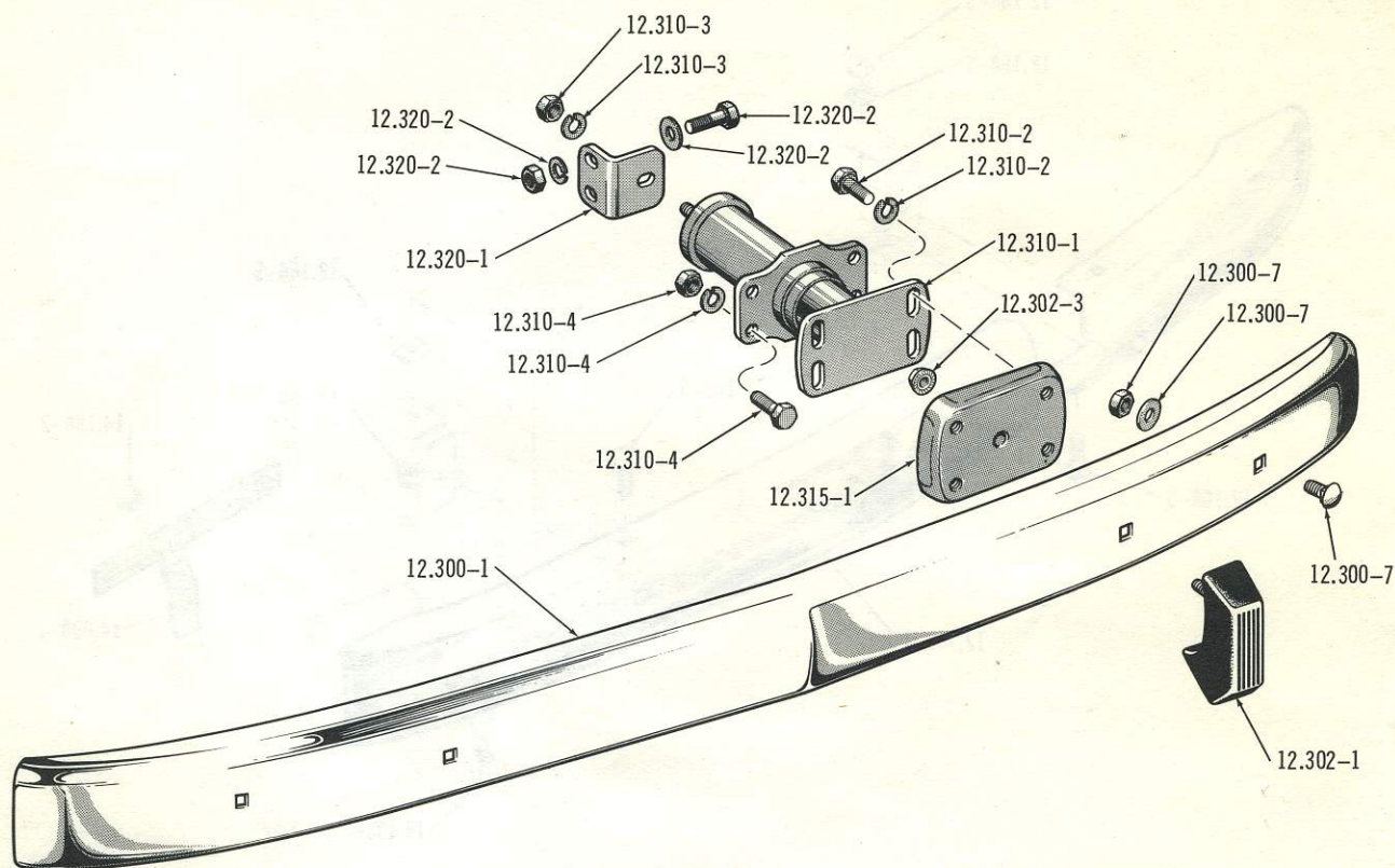
FRONT BUMPER . . . 1974 80 (WEAB)
