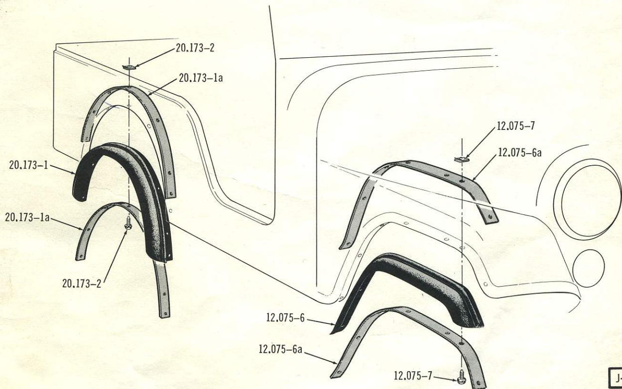
FENDER EXTENSION . . . 83-93 (RENEGADE)
