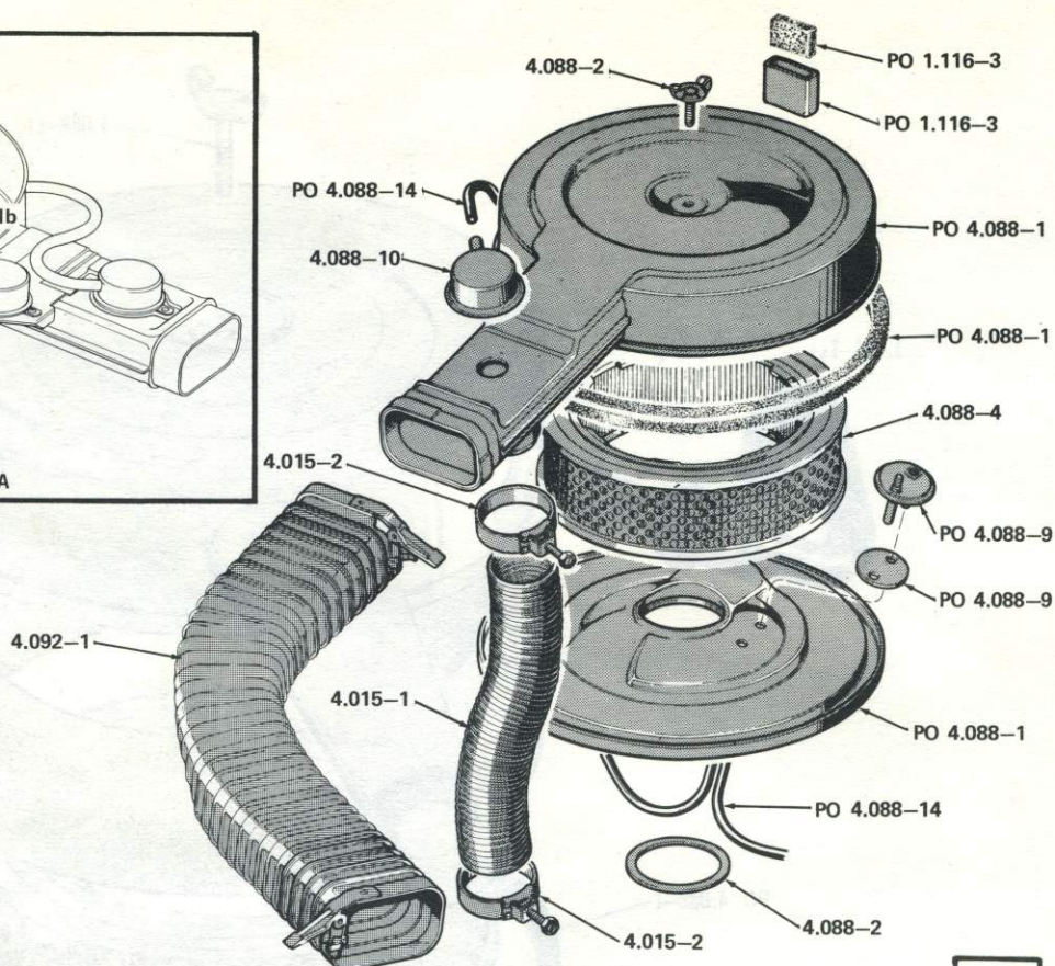
CARBURETOR AIR CLEANER . . . 1978/ 80-90 SIX (LPB)
