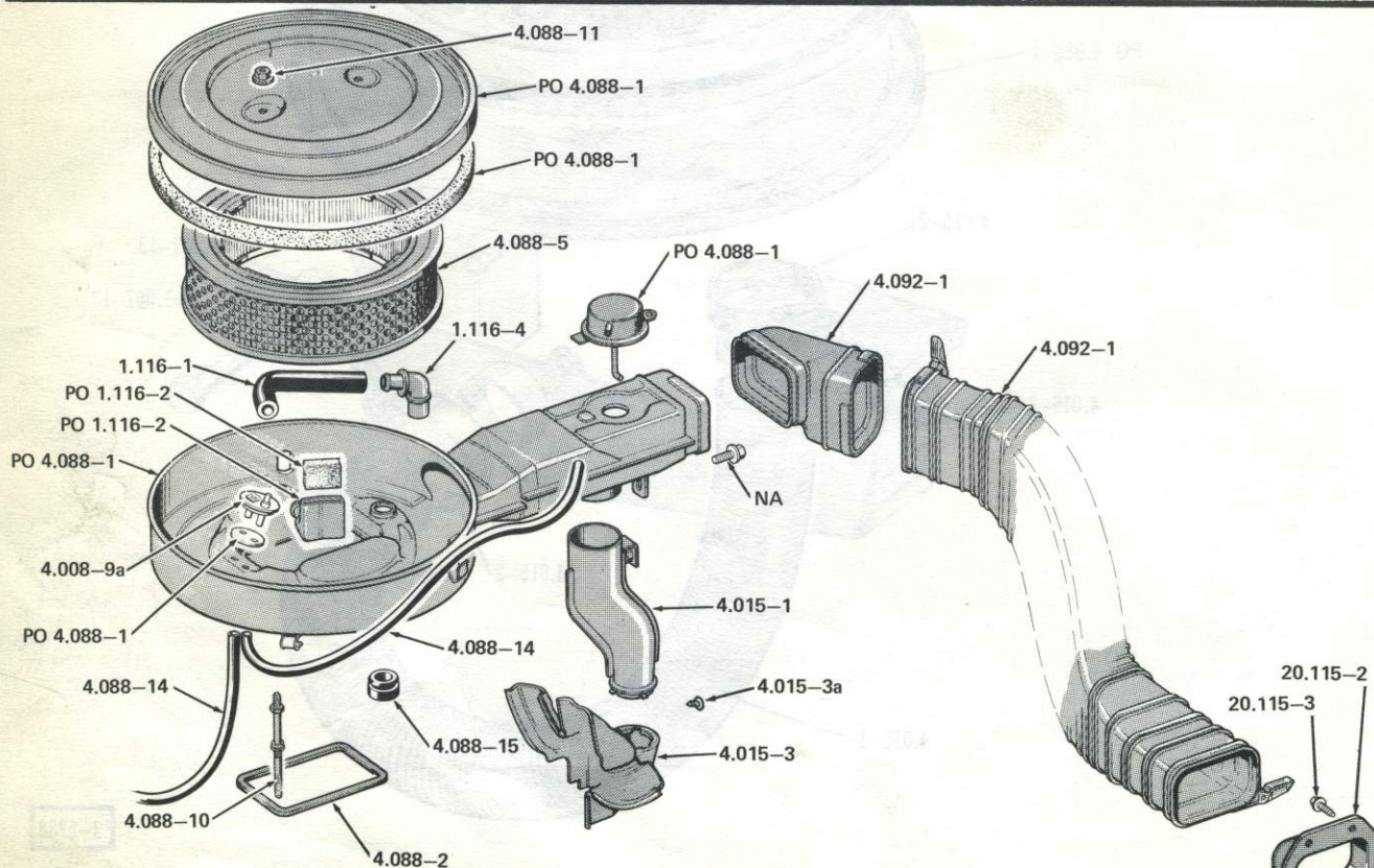
CARBURETOR AIR CLEANER . . . FOUR
