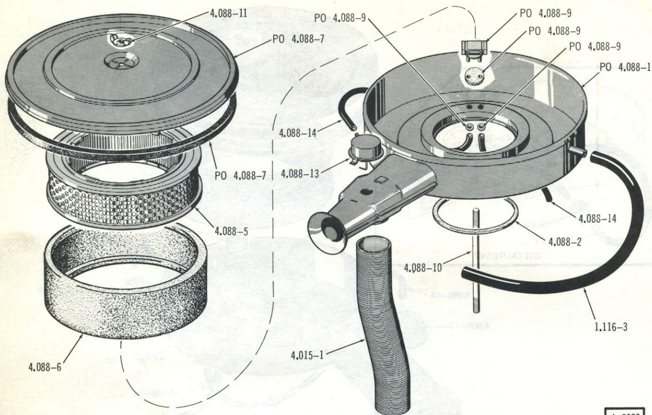
CARBURETOR AIR CLEANER . . . V8 (1974/1977)
