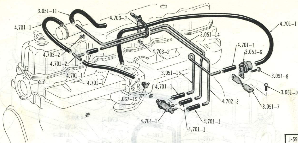
VACUUM ADVANCE MODULATION SYSTEM . . . 10-20-40 (SIX)
