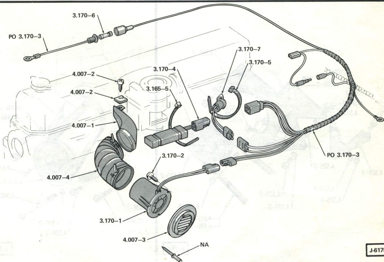
CARBURETOR COOLING FAN ... SIX (CALIFORNIA)
