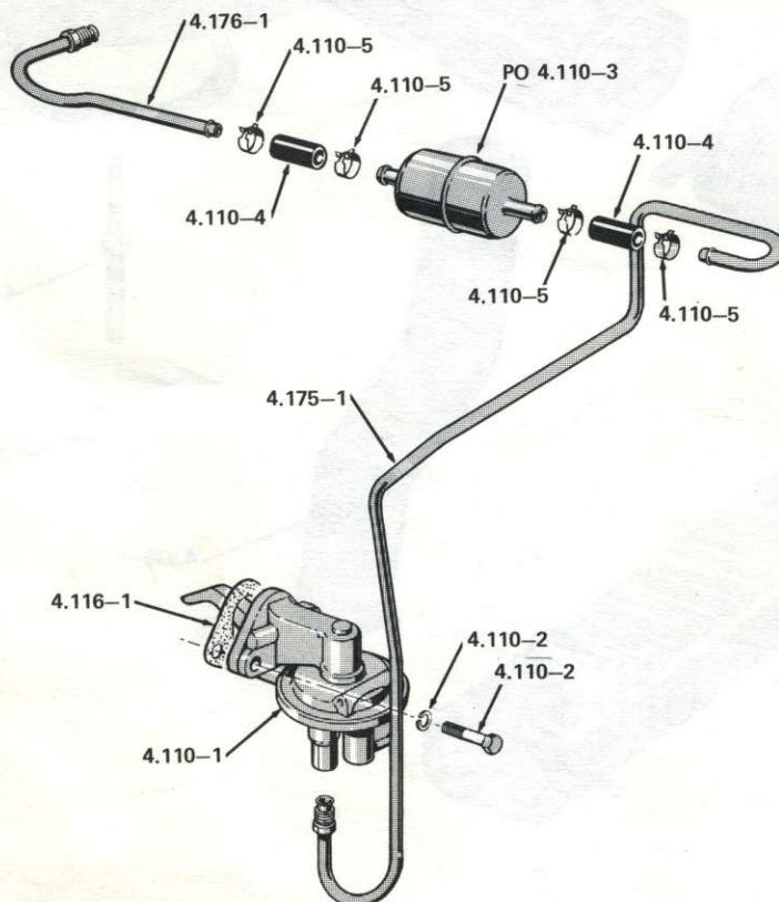
FUEL PUMP AND FUEL FILTER . . . SIX AND V8 (W/O FUEL RETURN LINE)
