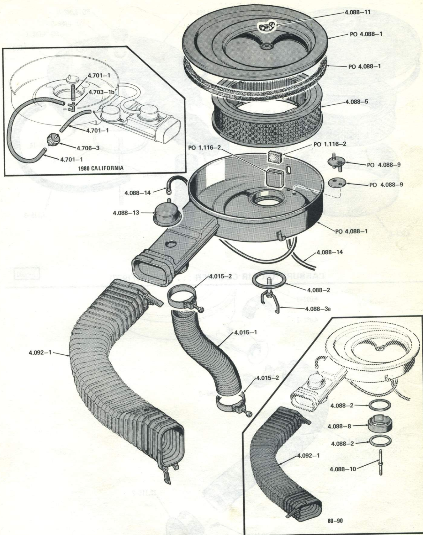
CARBURETOR AIR CLEANER . . . 1978/ SIX (WPB)
