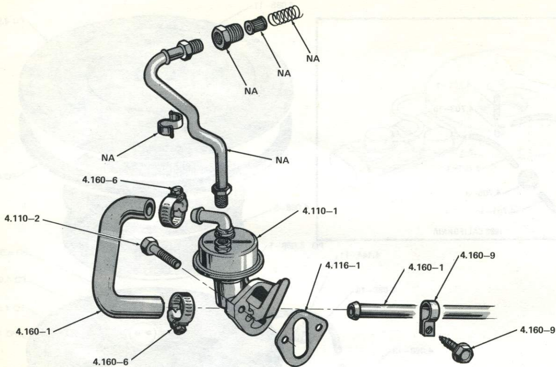
FUEL PUMP, FILTER AND LINES . . . 1980 (FOUR)
