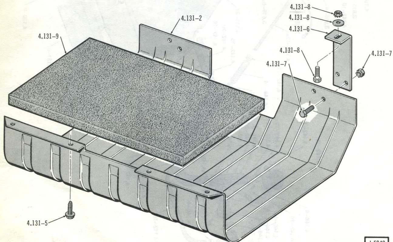
FUEL TANK SKID PLATE . . . 1974/1975 80
