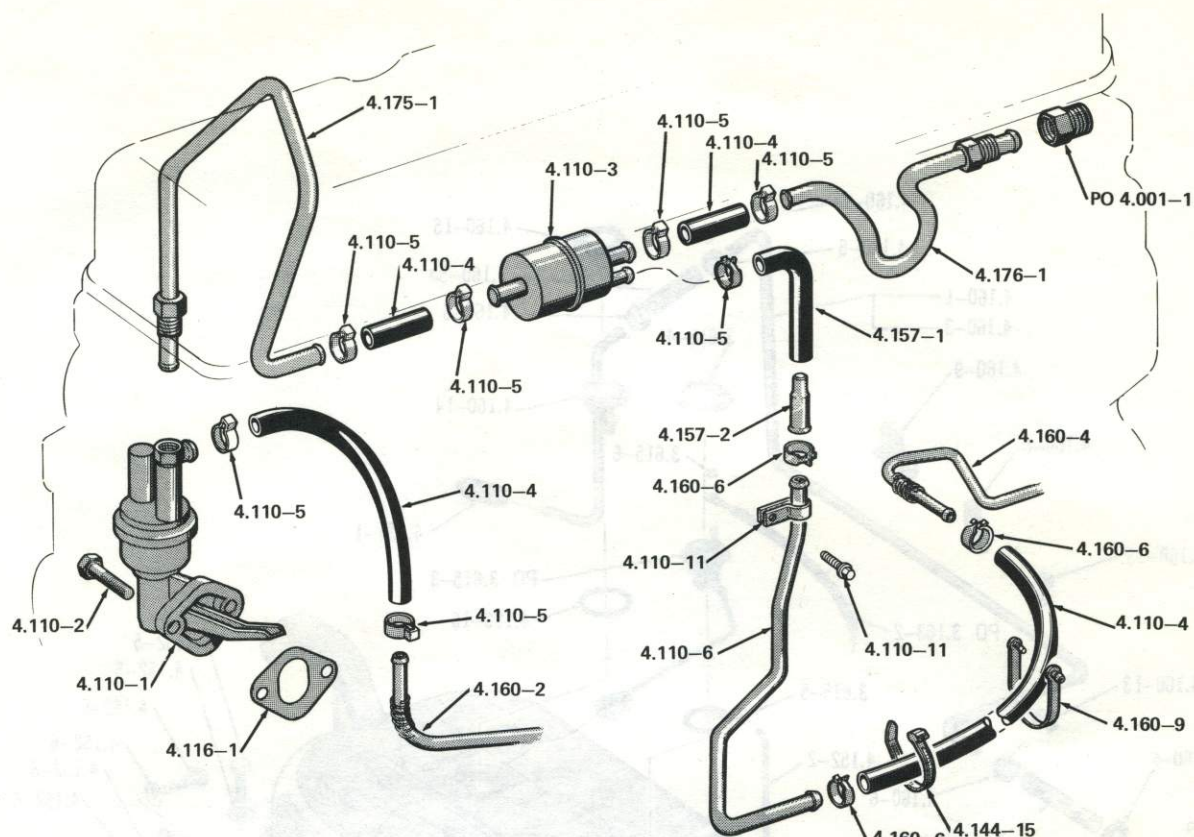
FUEL PUMP, FILTER AND LINES ... 1975/ SIX
