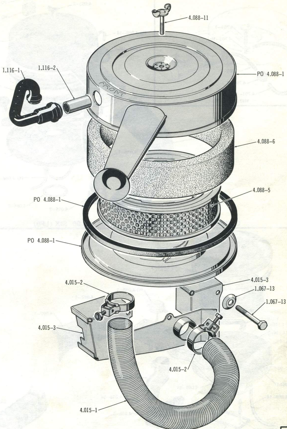
CARBURETOR AIR CLEANER . . . SIX (1974/1977)
