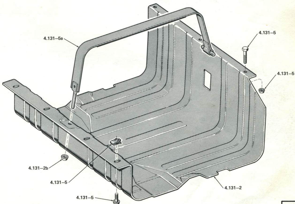
FUEL TANK SKID PLATE . . . 1976/ 80-90
