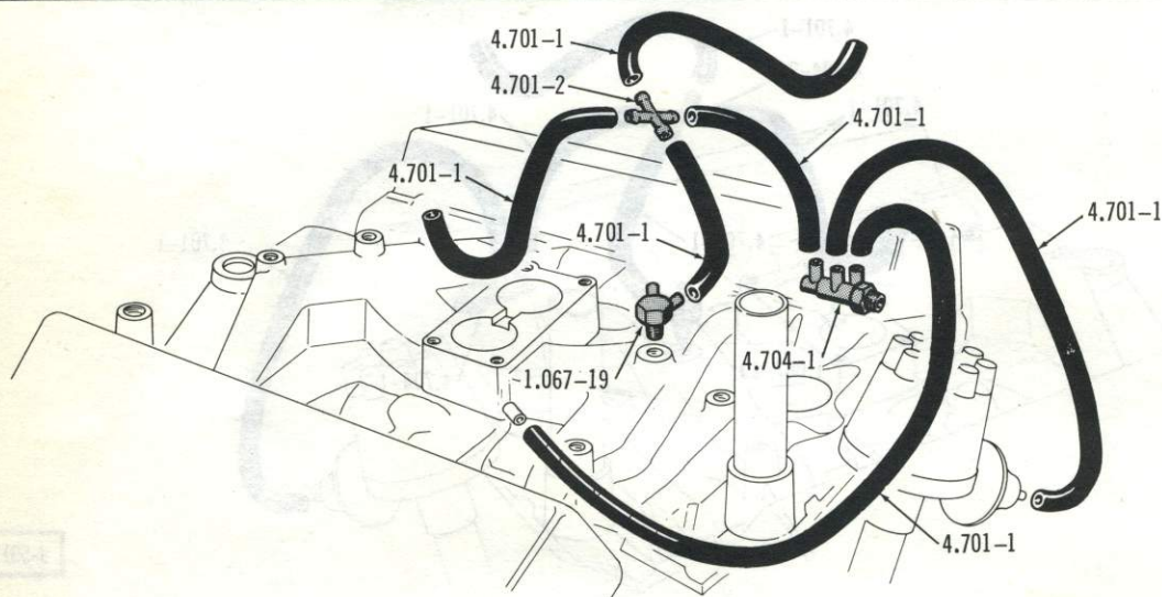
VACUUM ADVANCE MODULATION SYSTEM . . . 10-25-45 (401-E/CALIF), 26-46 (V8-WHDC)
