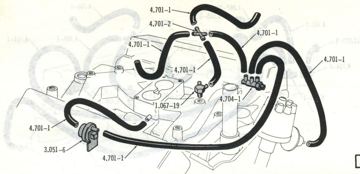
VACUUM ADVANCE MODULATION SYSTEM . . . 10-25-45 (360-WHDC-E/CALIF), 1974 80 (V8-E/CALIF), 1975 80 (V8-CALIF)
