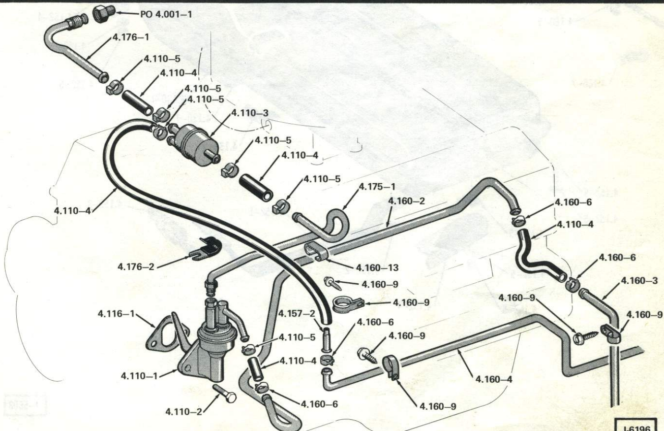
FUEL PUMP, FILTER AND LINES ... 1975/ V8
