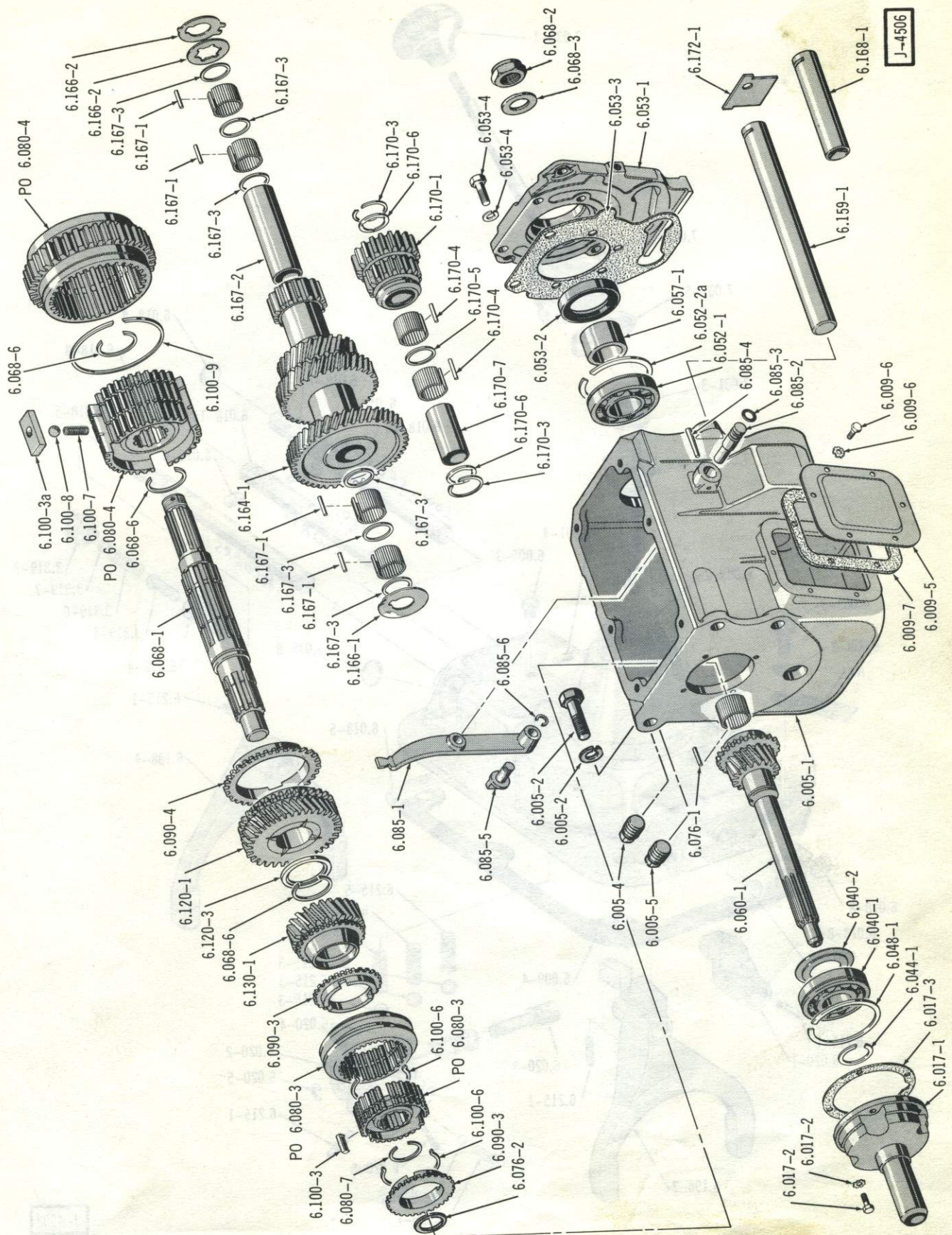
TRANSMISSION ASSEMBLY (W4ST) ... T18
