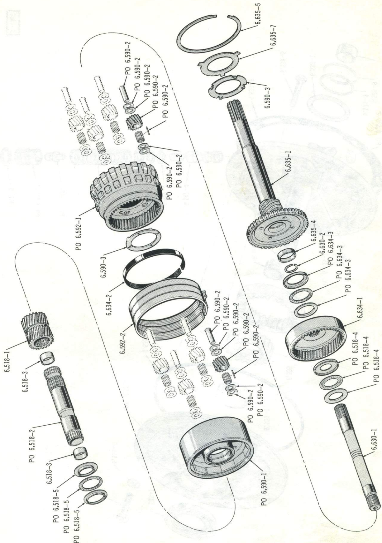
HYDRAMATIC PLANET CARRIER . . . 1974/1979
