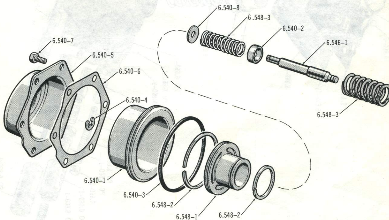
HYDRAMATIC FRONT SERVO . . . 1974/1979
