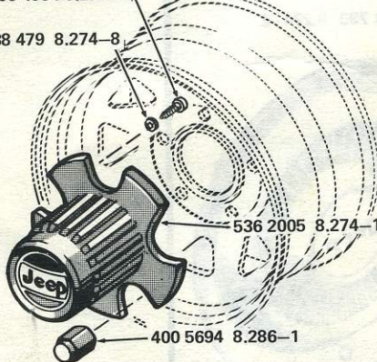
HUB CAP (WITH CUSTOM STEEL WHEEL - 8 SLOTTED) . . . 1980 83-93 (REAR WHEELS ONLY)
