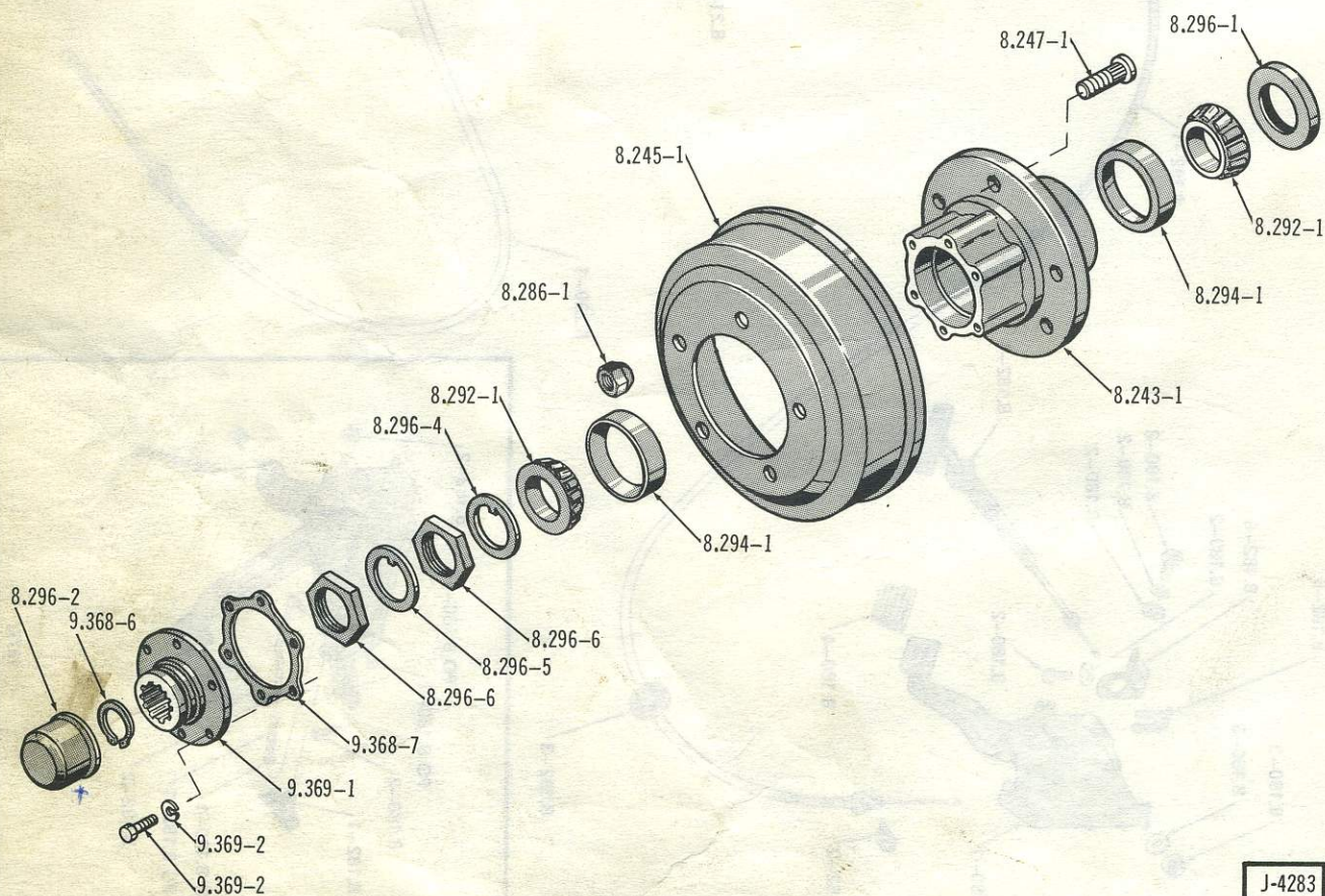
FRONT HUB AND DRUM . . . 80-90 (LDB)
