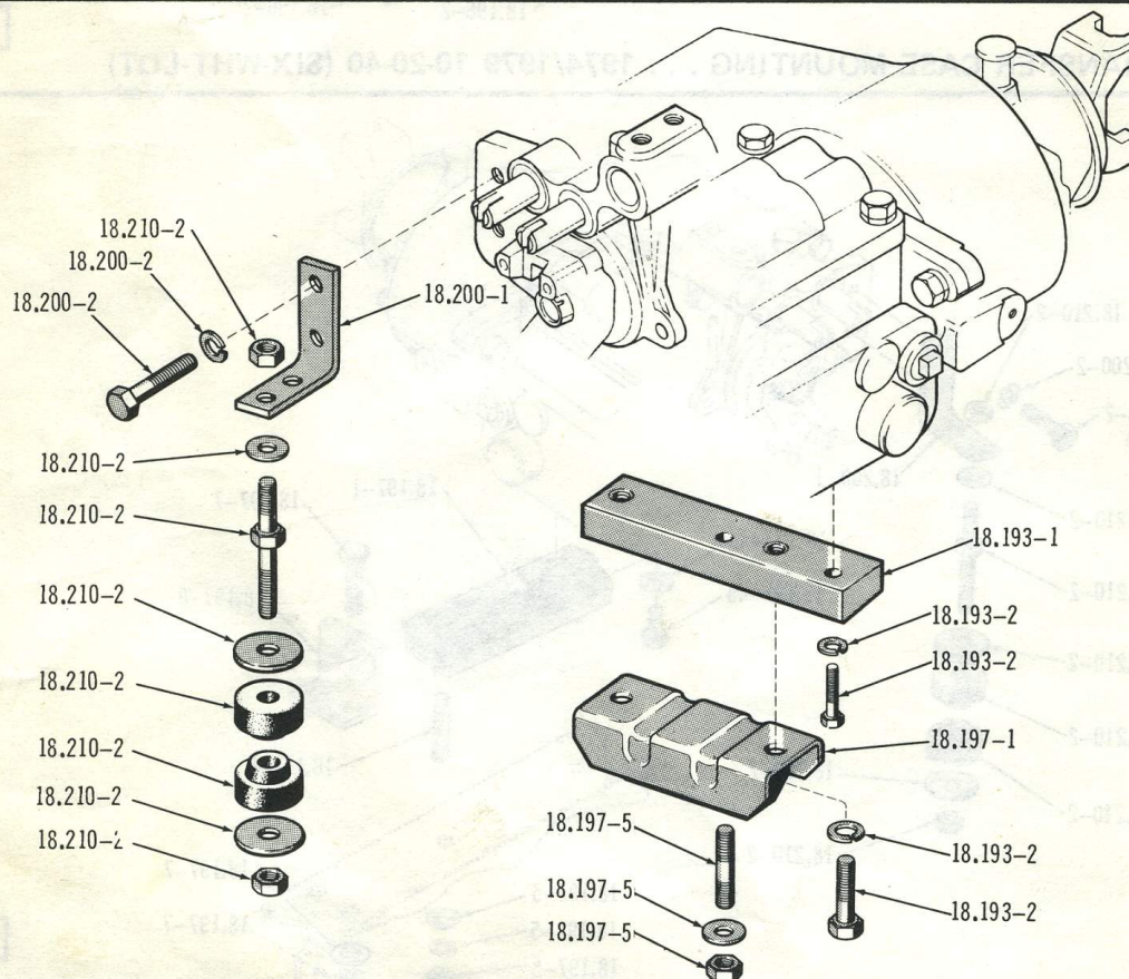
TRANSFER CASE MOUNTING . . . 1974/1979 10-20-40 (V8-WHT-LQT)
