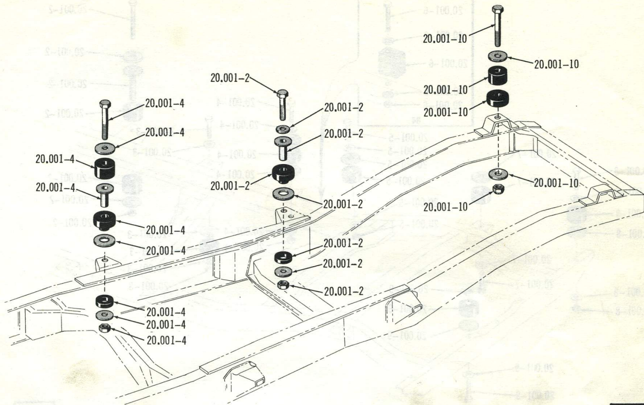
BODY HOLD DOWN PARTS . . . 1974/1975 20-40
