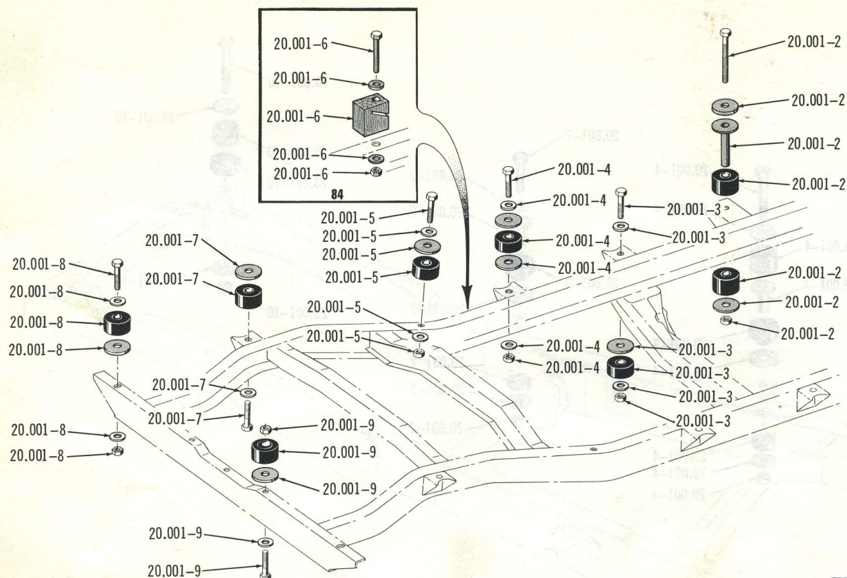
BODY HOLD DOWN PARTS . . . 1974/1975 80
