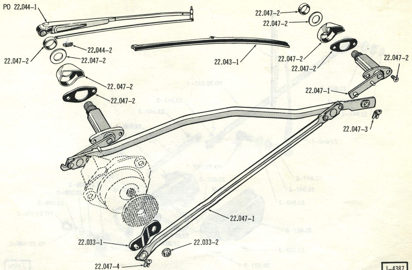
WINDSHIELD WIPER ARMS AND BLADES . . . 10-20-40
