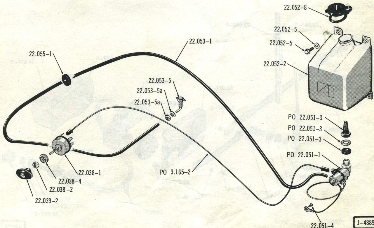
ELECTRIC OPERATED WINDSHIELD WASHERS . . . 80-90
