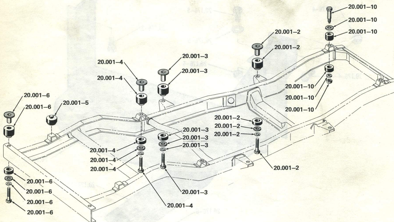
BODY HOLD DOWN PARTS ... 1974/1975 10
