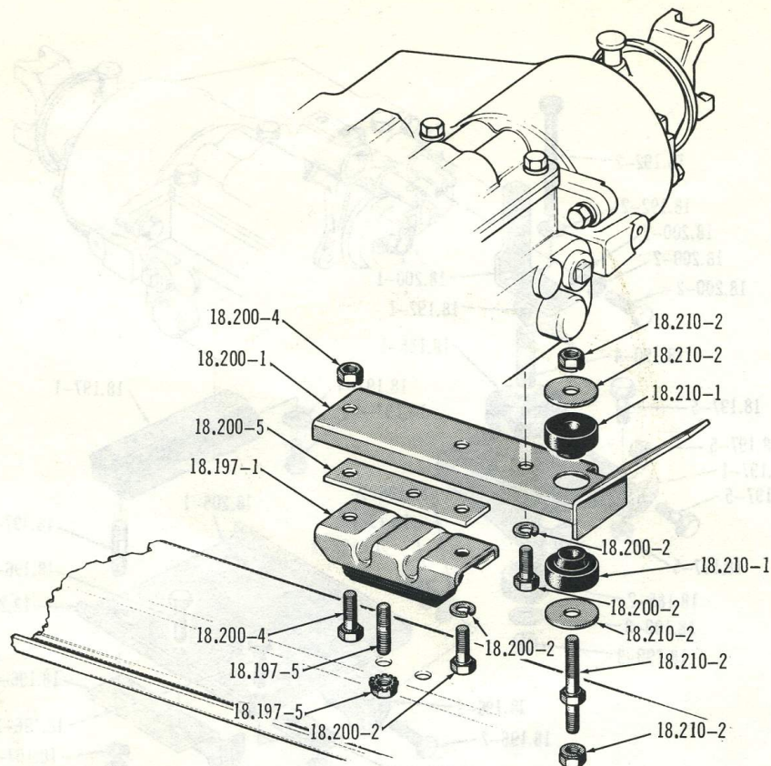
TRANSFER CASE MOUNTING . . . 1974/1979 10-20-40 (SIX-WMT) (V8-W3ST) (V8-WHT-WQT)
