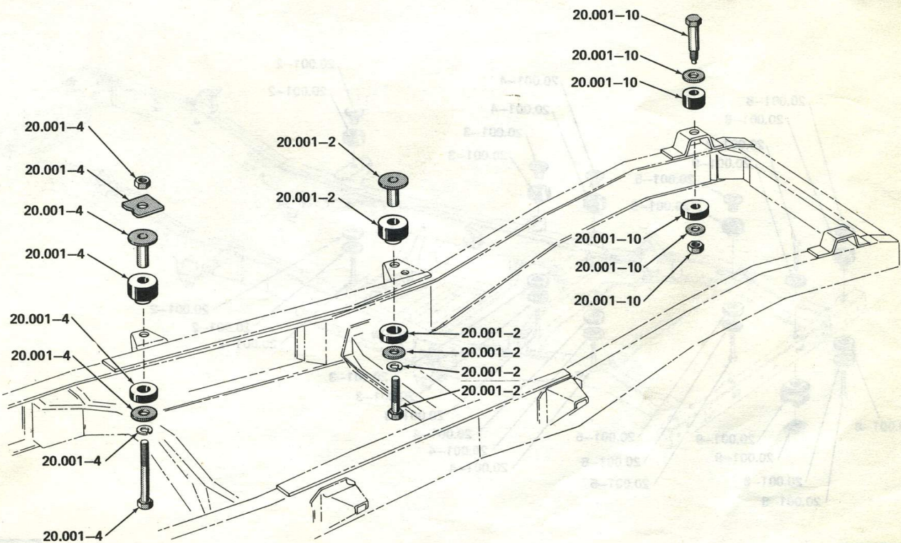
BODY HOLD DOWN PARTS . . . 1974/1975 20-40
