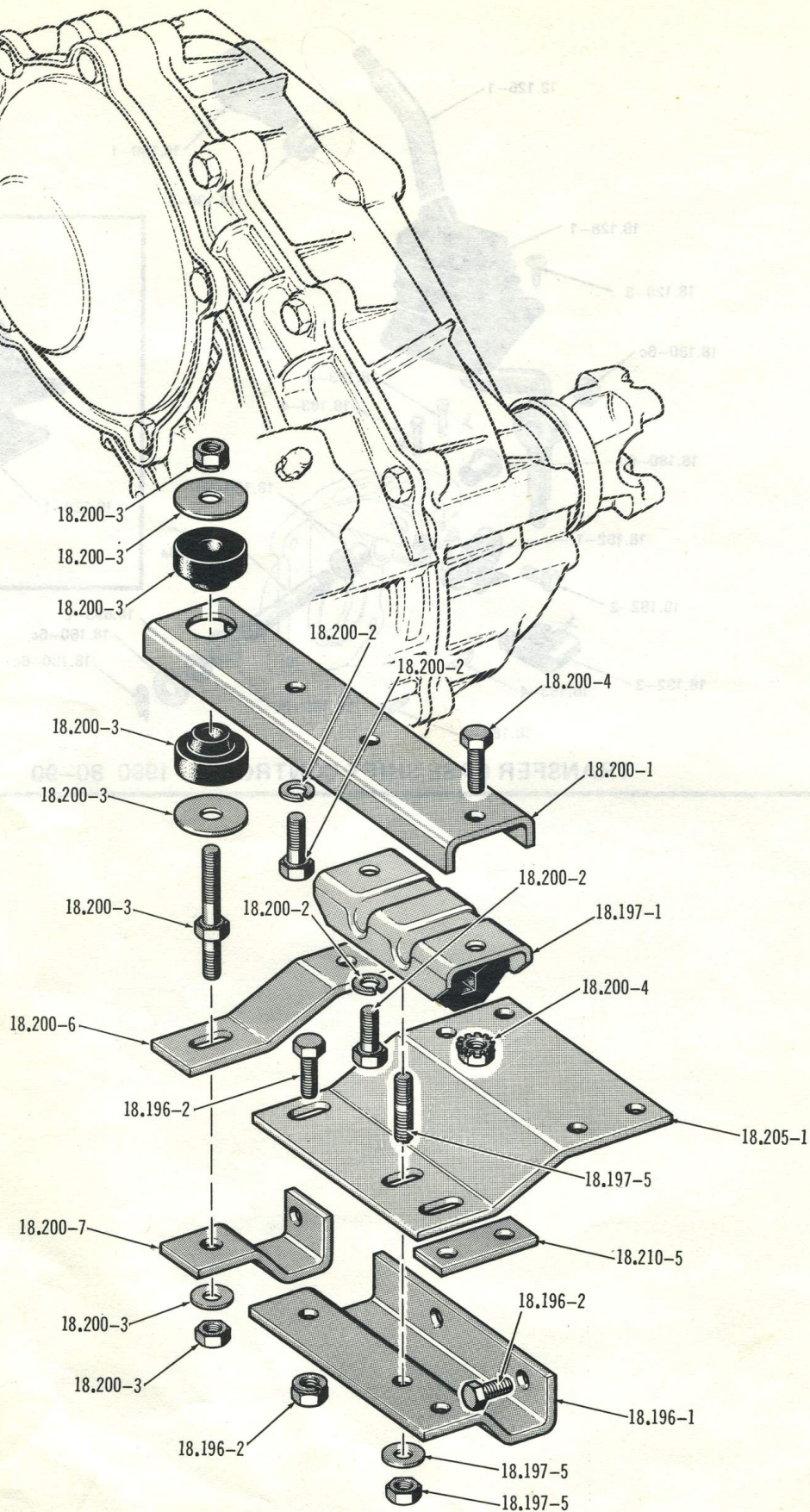
TRANSFER CASE MOUNTING . . . 1974/1979 10-20-40 (SIX-WHT-WQT)
