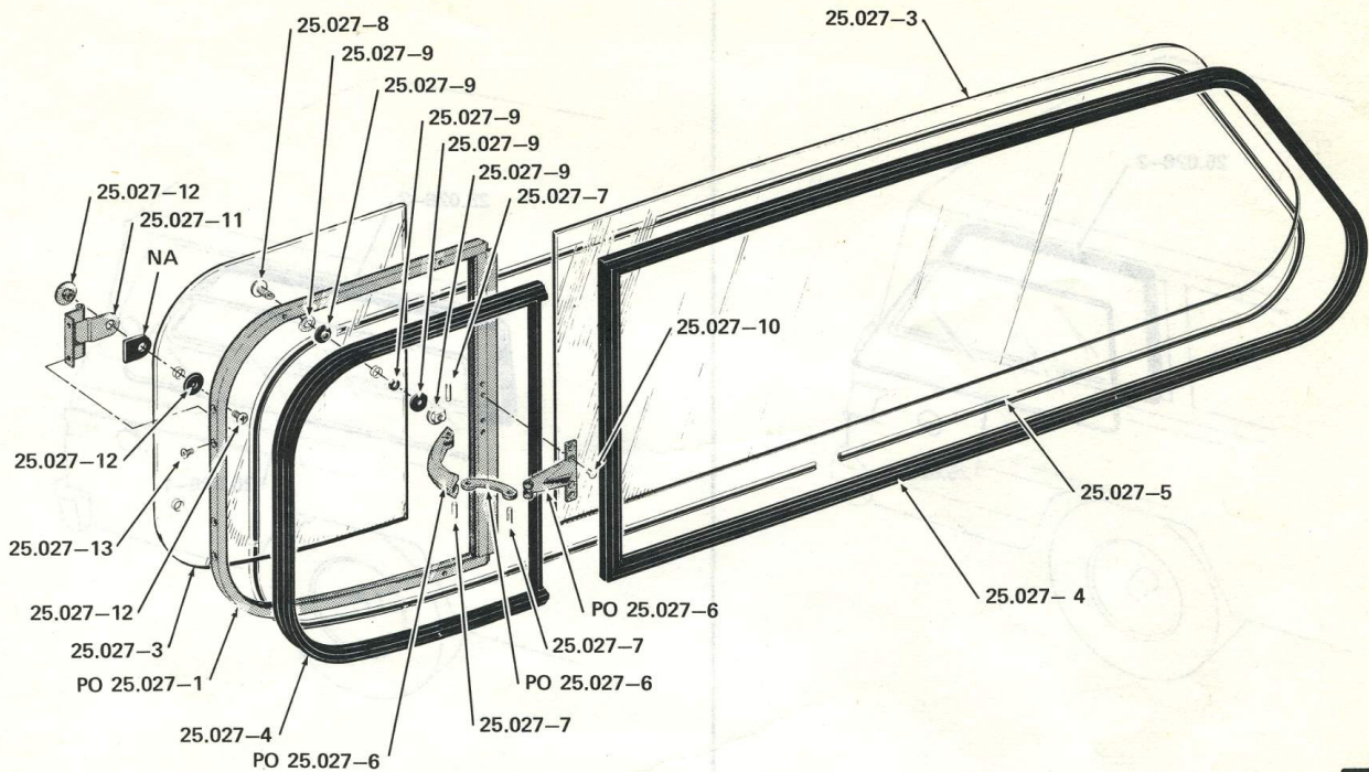
REAR QUARTER PIVOTING WINDOW . . . 1974/1978 16-17
