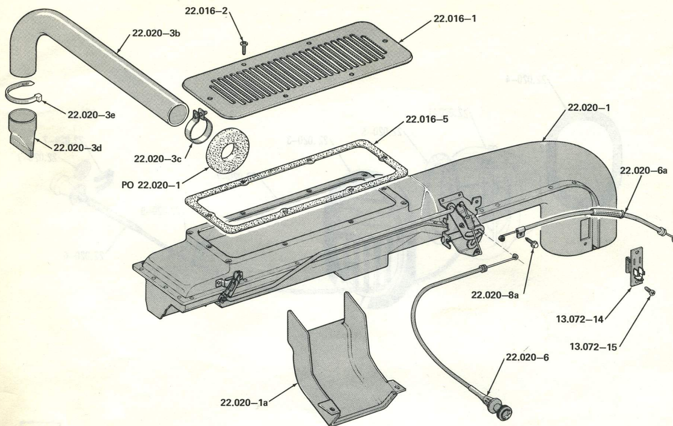
COWL FRESH AIR INTAKE ... 1977/ 80-90
