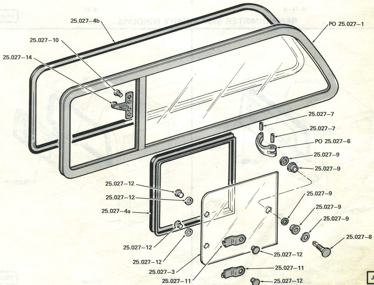
REAR QUARTER PIVOTING WINDOW . . . 1979/ 16-17
