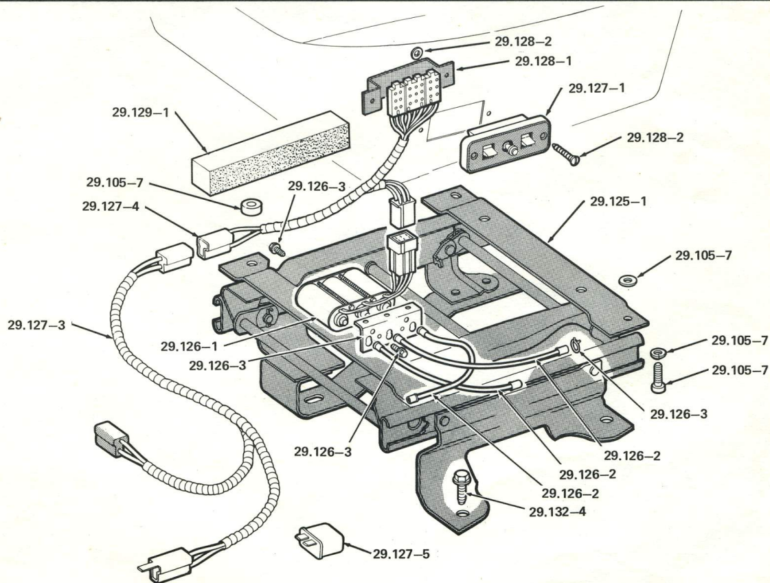
FRONT SEAT ADJUSTING SLIDE...WITH POWER OPTION
