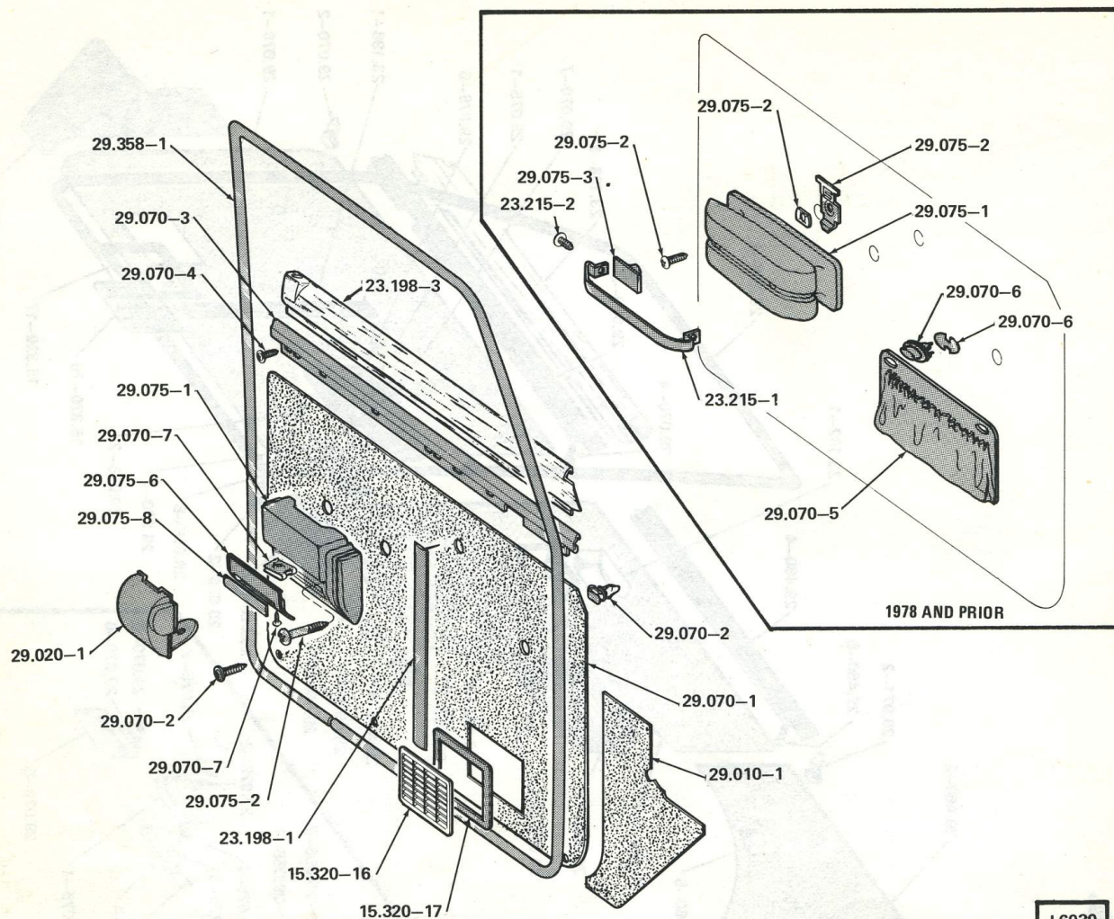
INTERIOR TRIM PANELS . . . 20-40
