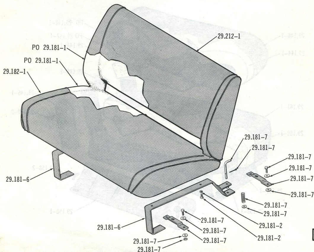
REAR PASSENGER SEAT ... 1974/1975 80
