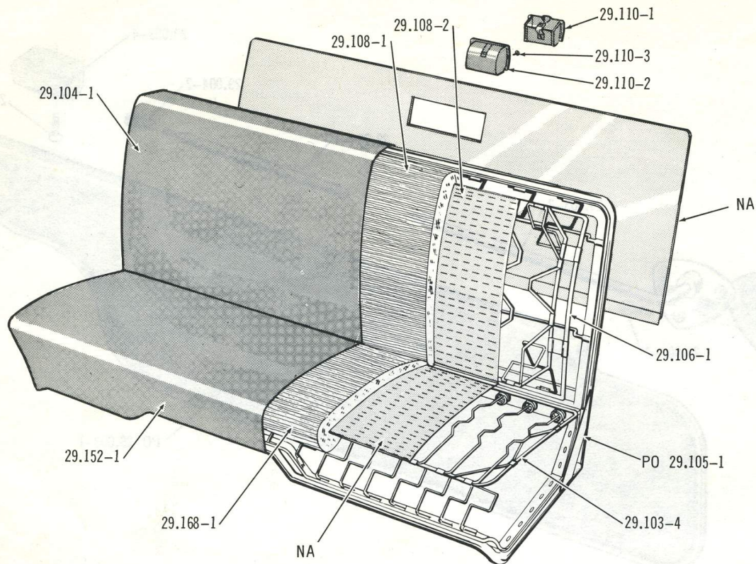
ONE-PIECE FRONT SEAT ... 14-15-18
