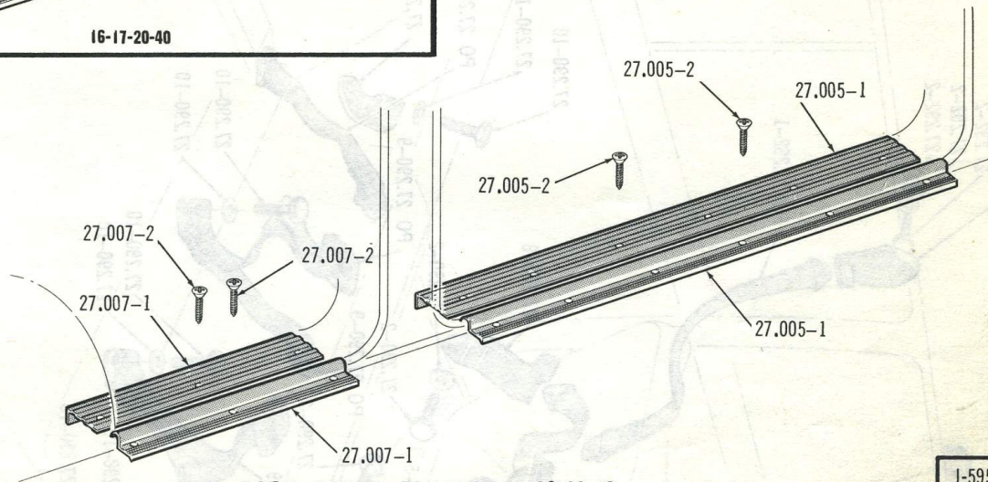
DOOR SCUFF PLATES... 10-20-40
