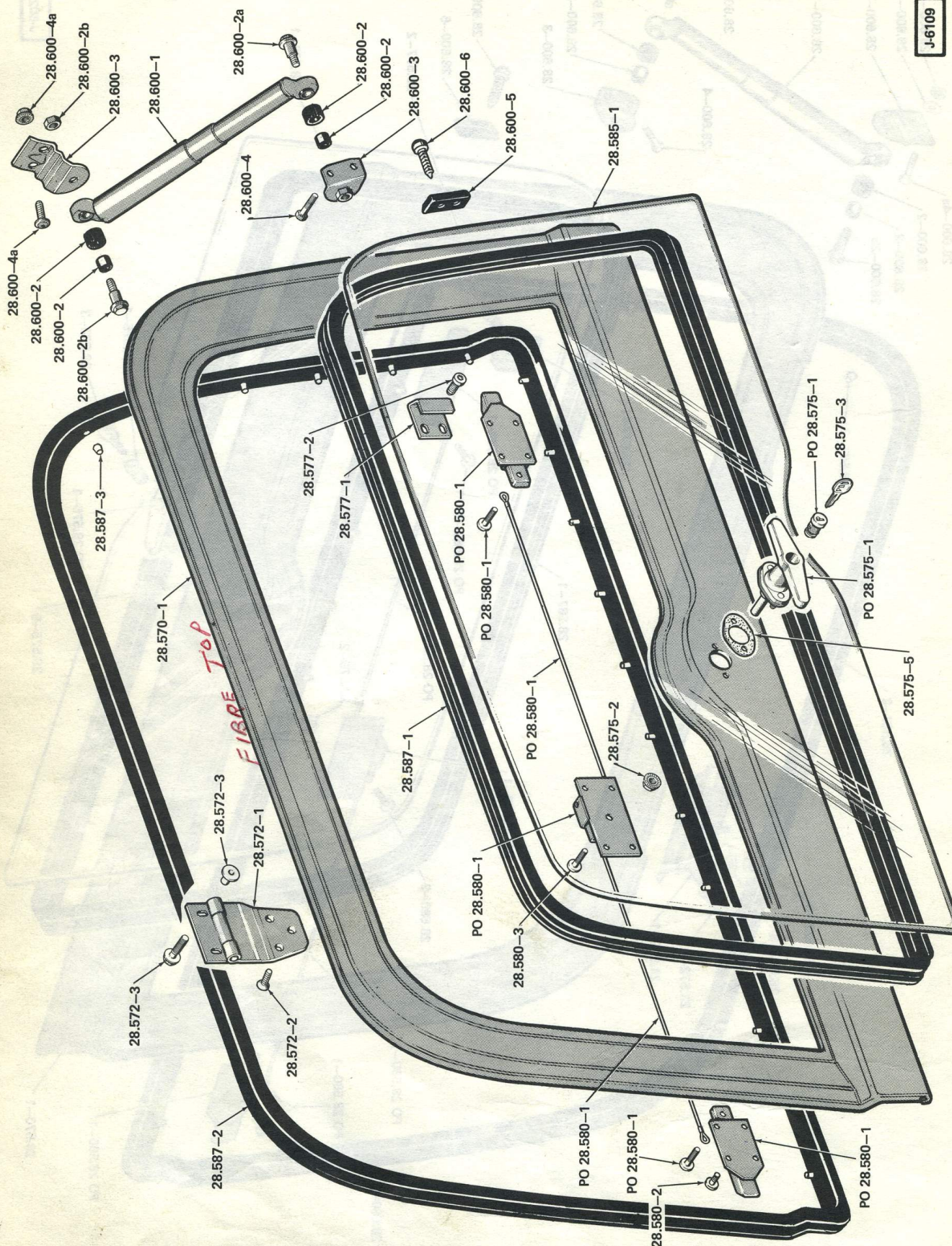
LIFTGATE . . . 90 (WITH FULL TOP ENCLOSURE – TYPE 2)
