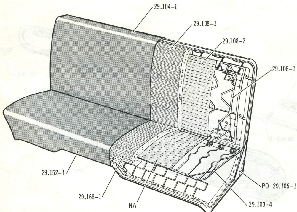
ONE-PIECE FRONT SEAT ... 14-15-18
