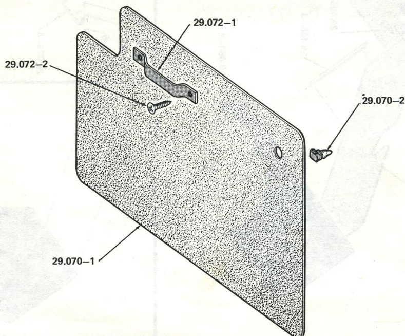
INTERIOR TRIM PANELS . . . 90 (WITH FULL TOP ENCLOSURE)
