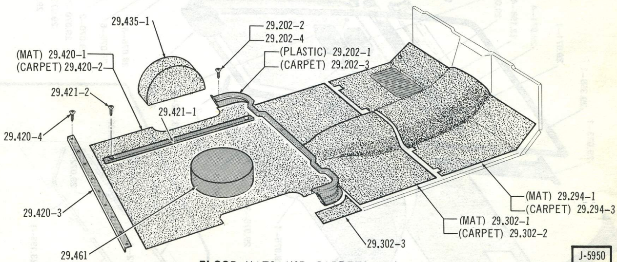
FLOOR MATS AND CARPETS . . . 10
