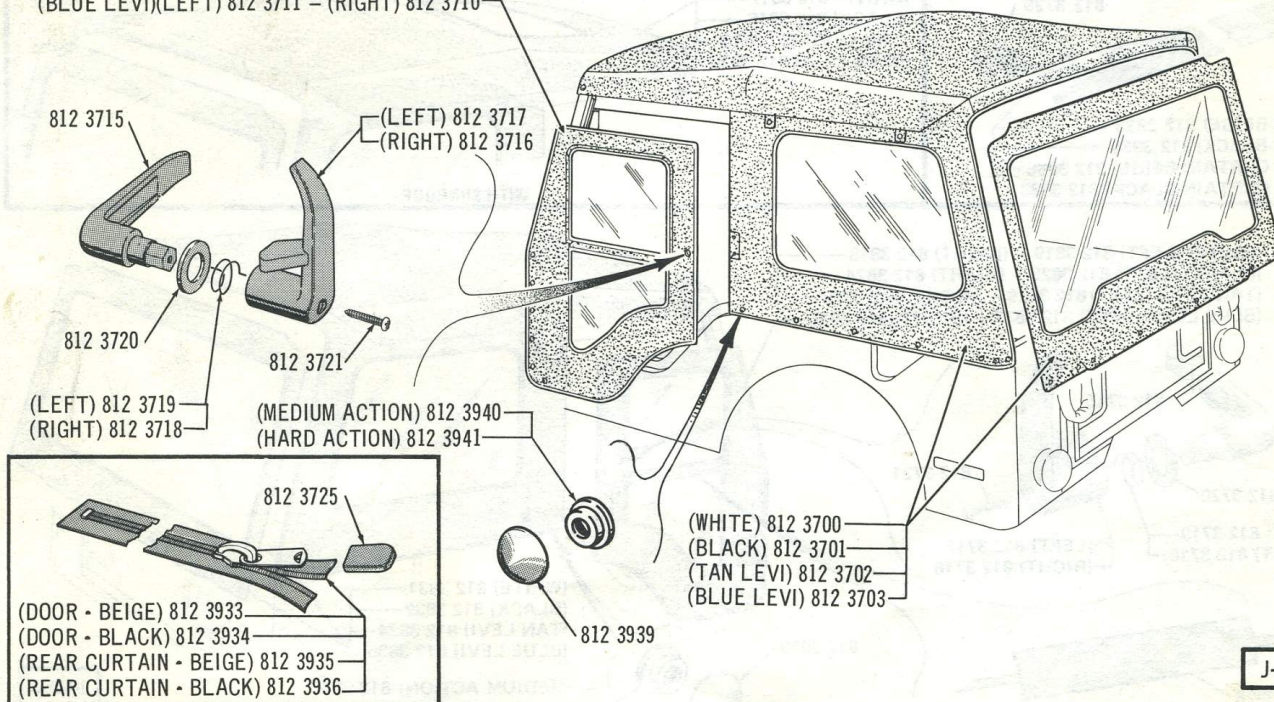
CANVAS TOP (SAFARI) - 3100 SERIES ... 1974/1975 83
