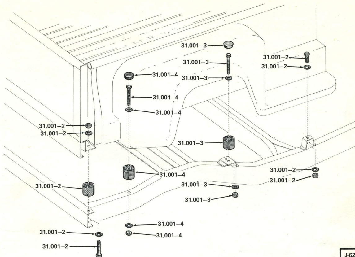
PICKUP BOX HOLD DOWN PARTS . . . 1980 25 (THRIFTSIDE)
