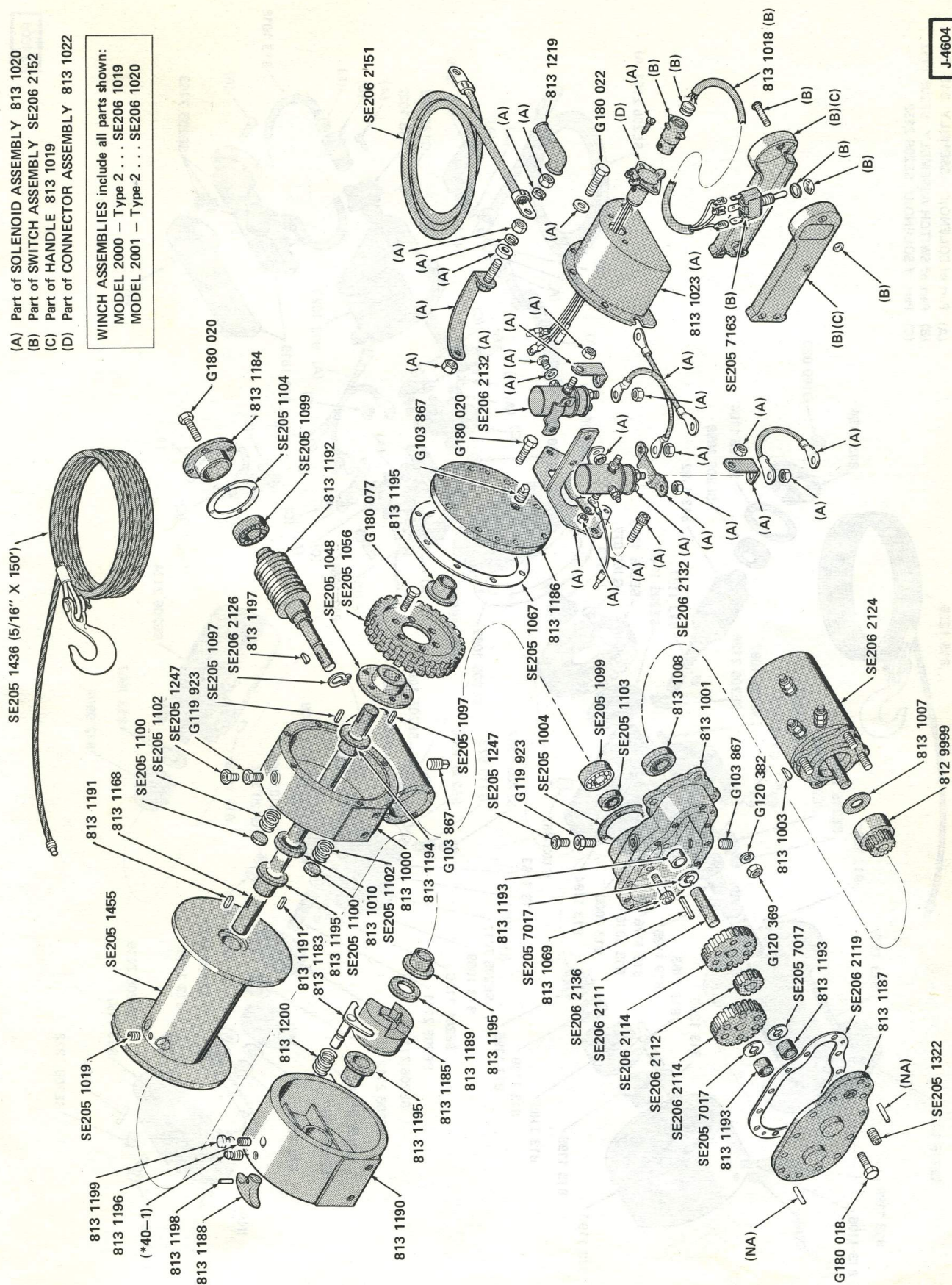
WINCH ASSEMBLY . . . RAMSEY ELECTRICAL (MODELS 2000 - TYPE 2 and 2001 - TYPE 2)
