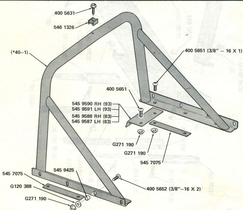
ROLL BAR . . . 83-93 (1974/1978, 1979 TYPE 1)
