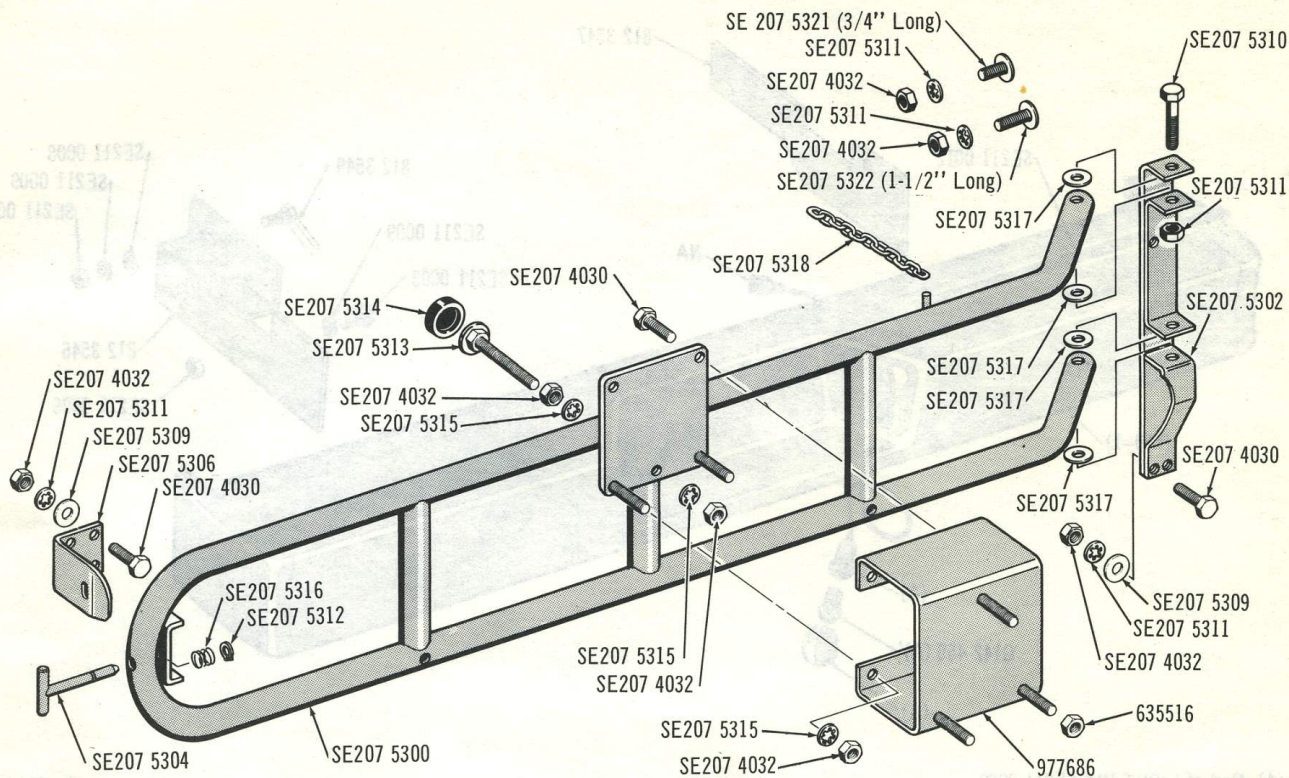
SPARE TIRE MOUNTING (SWING OUT) . . . 1974/1975 80
