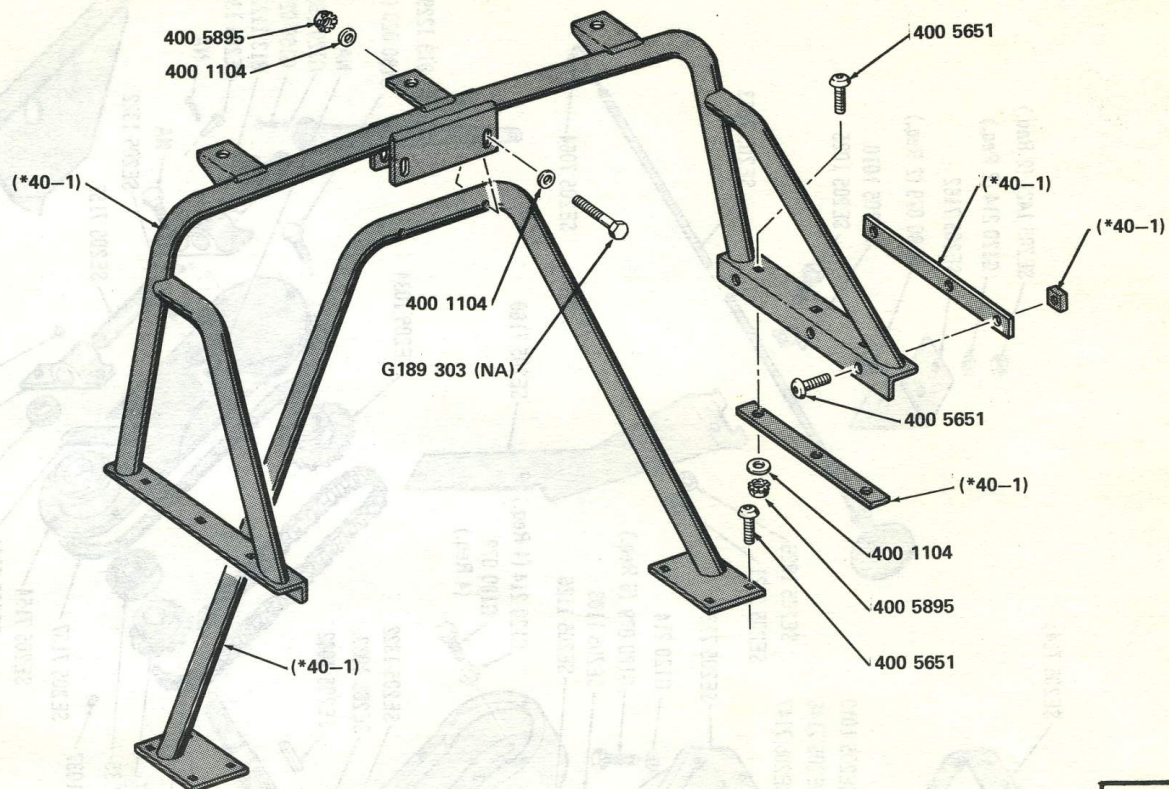
ROLL BAR . . . 20-40 (TOWNSIDE)
