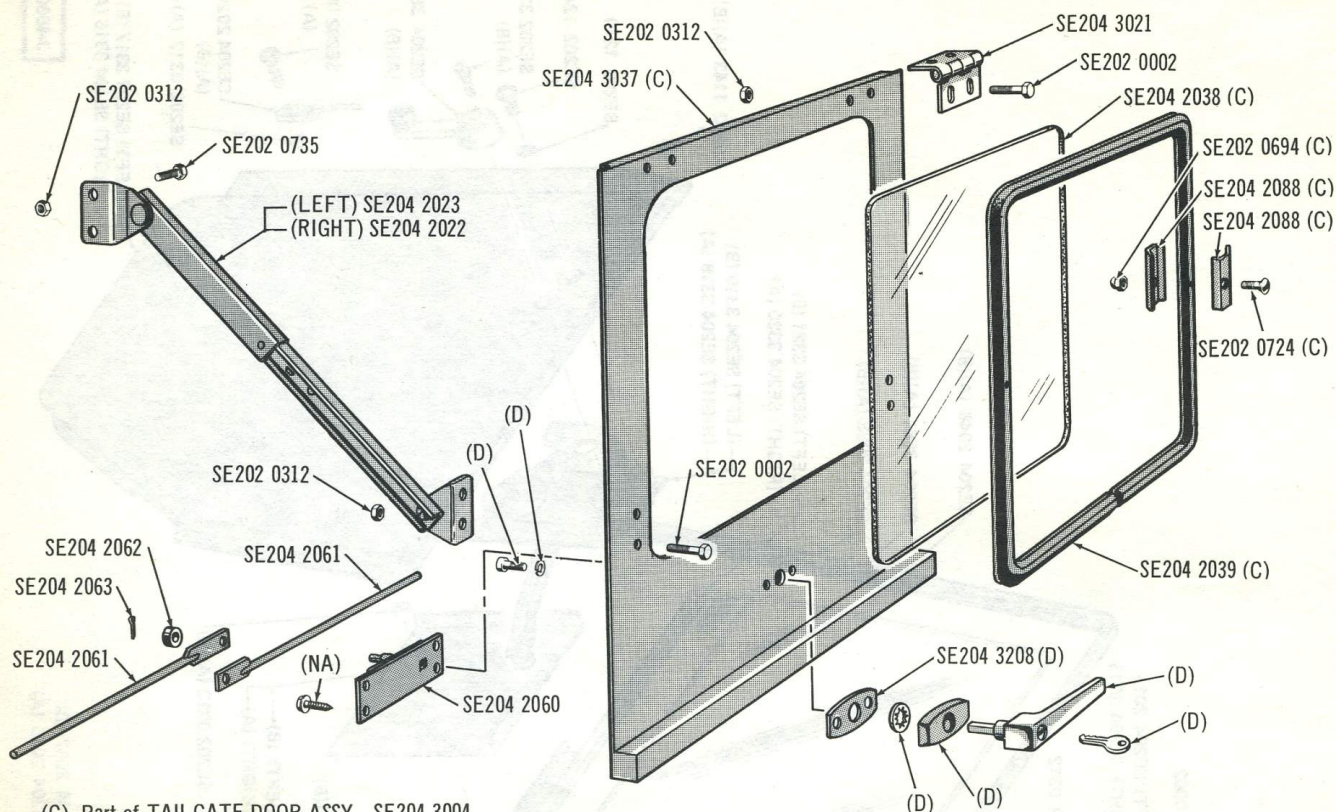
METAL CAB LIFTGATE ... 1974/1975 80
