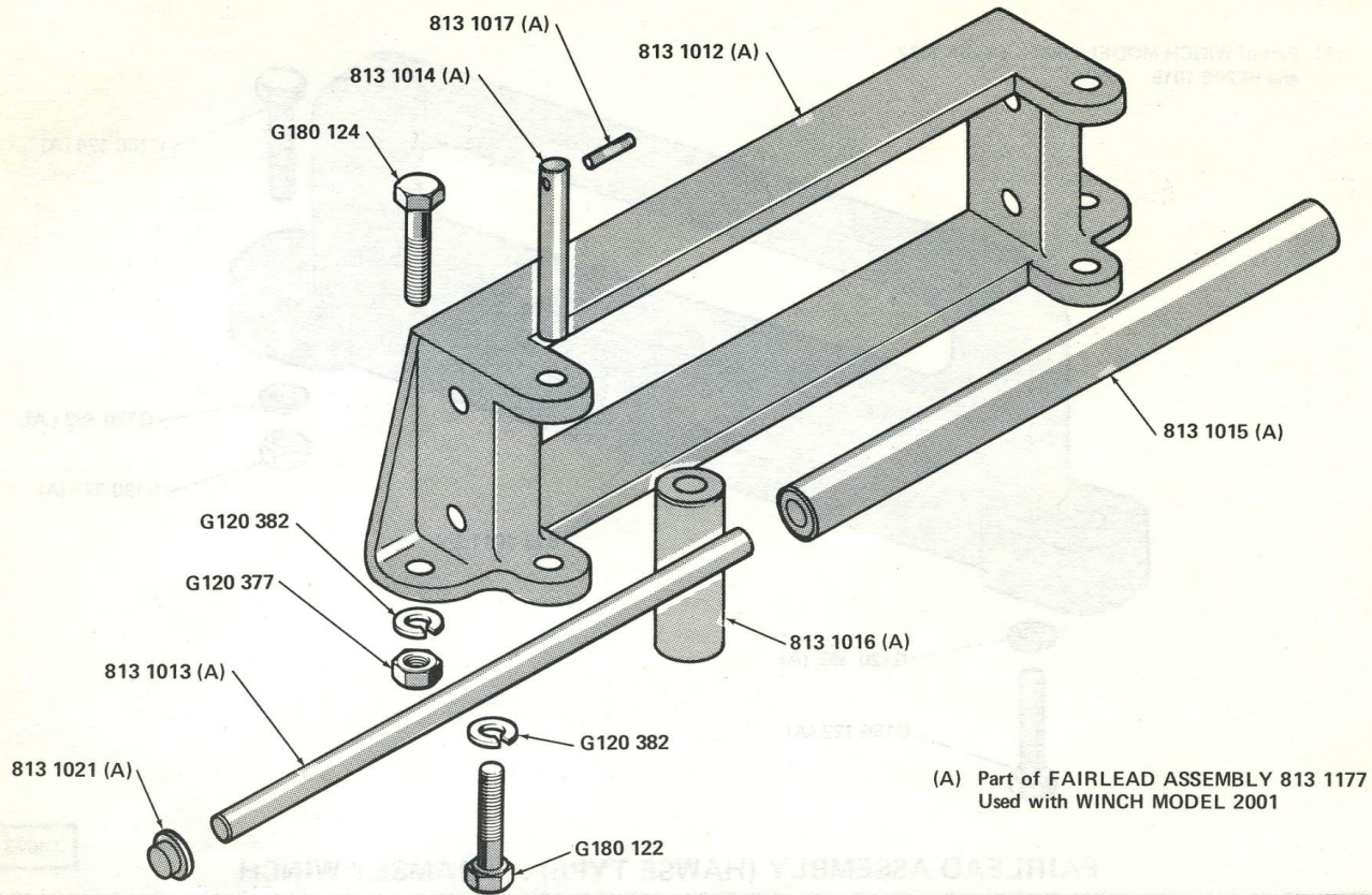
FAIRLEAD ASSEMBLY (ROLLER TYPE 2) – RAMSEY WINCH
