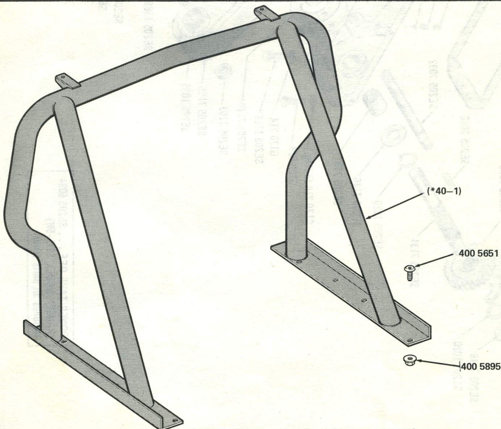
ROLL BAR . . . 20 (THRIFTSIDE)
