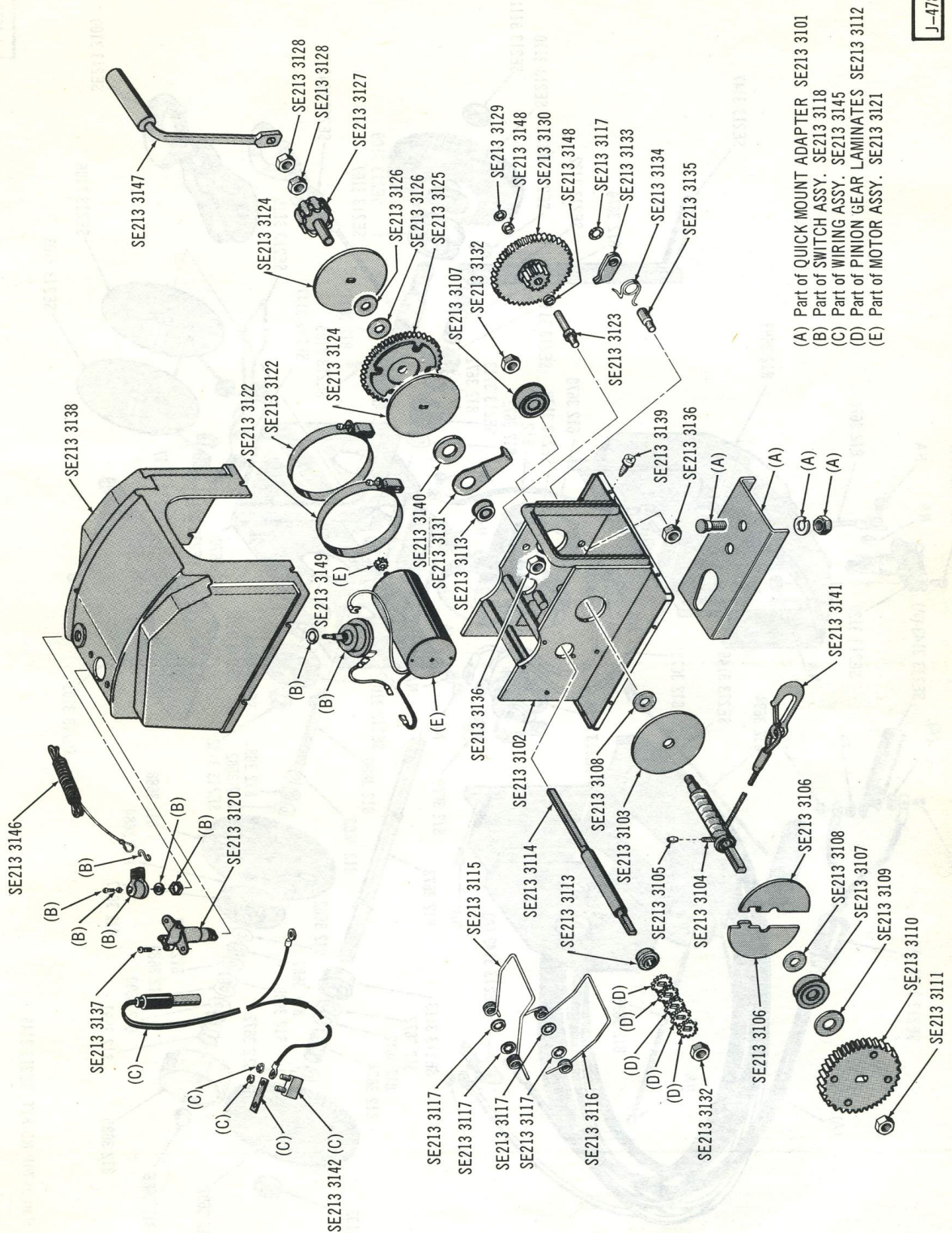
WINCH ASSEMBLY . . . PORTABLE ELECTRIC (MODEL A15-12) (MODEL A30-12C)
