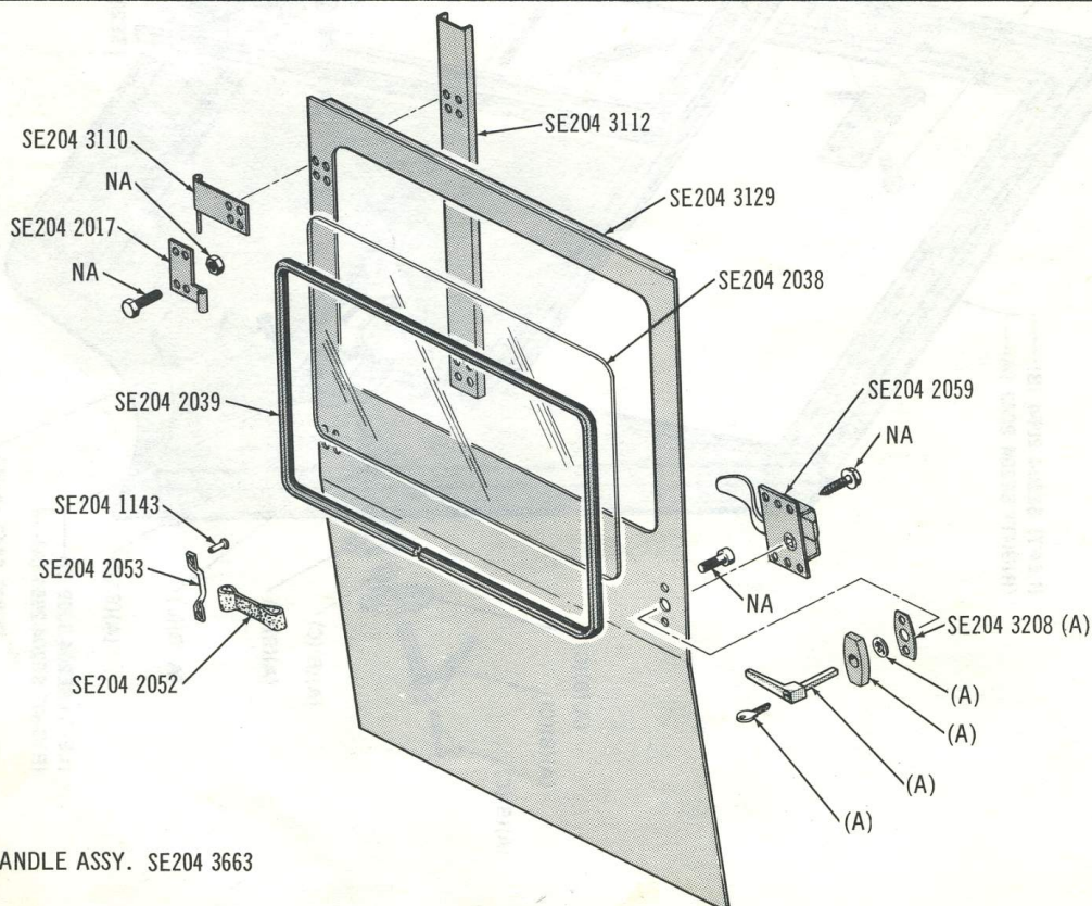
METAL CAB VERTICAL REAR DOOR ... 1974/1975 80
