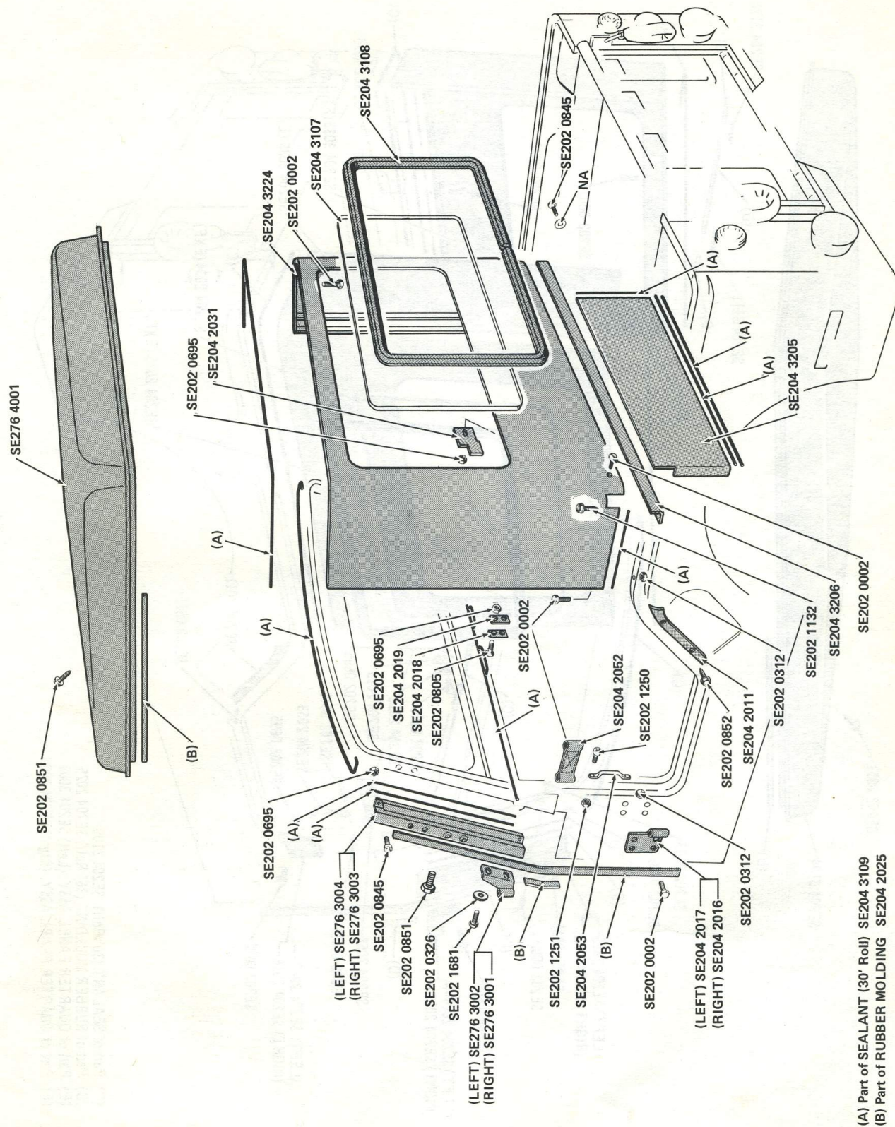
METAL CAB (HALF) . . . 1976/80
