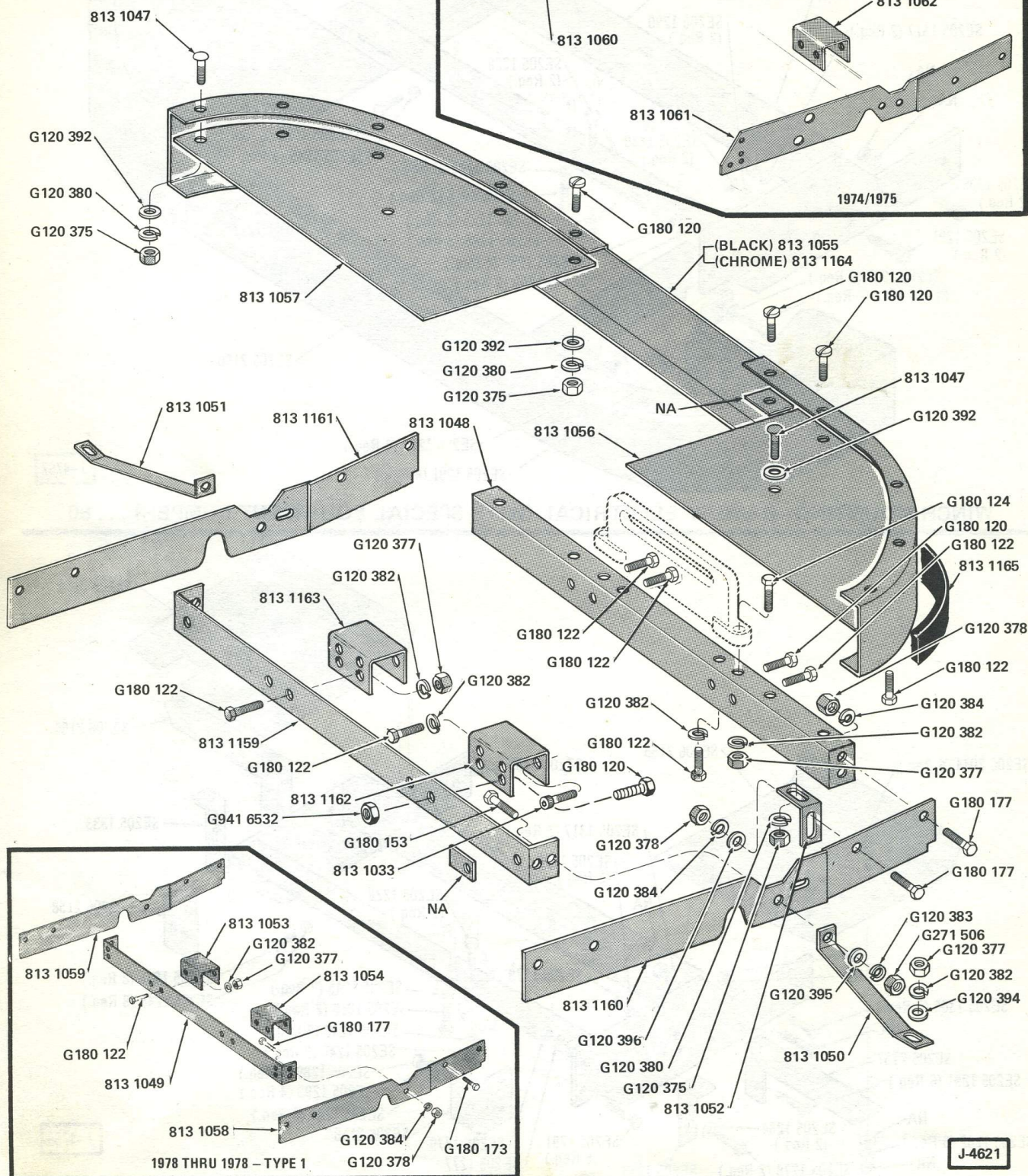
WINCH MOUNTING (RAMSEY) ... 1974/1978 10-20-40
