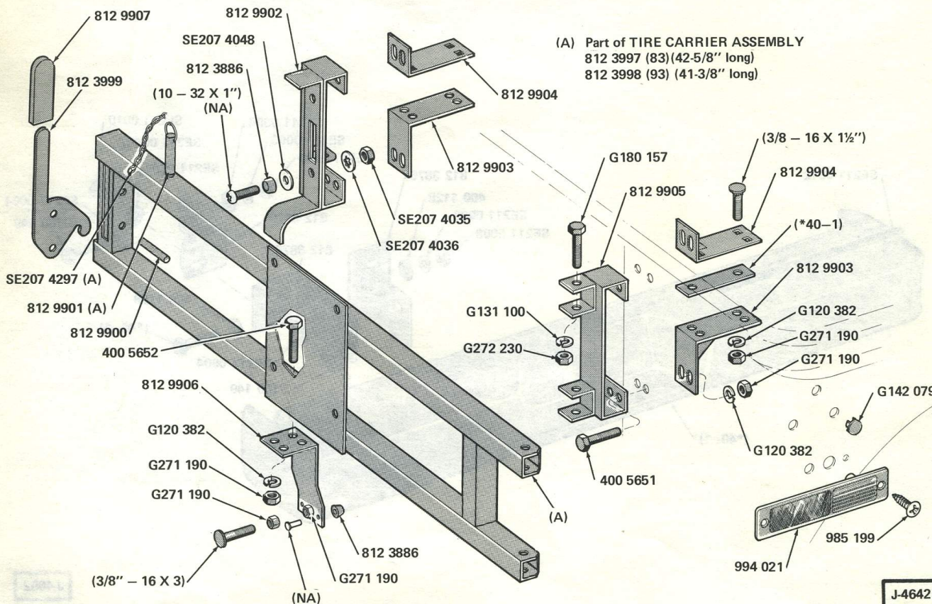
SPARE TIRE MOUNTING (SWING OUT) . . . 1978/ 80-90
