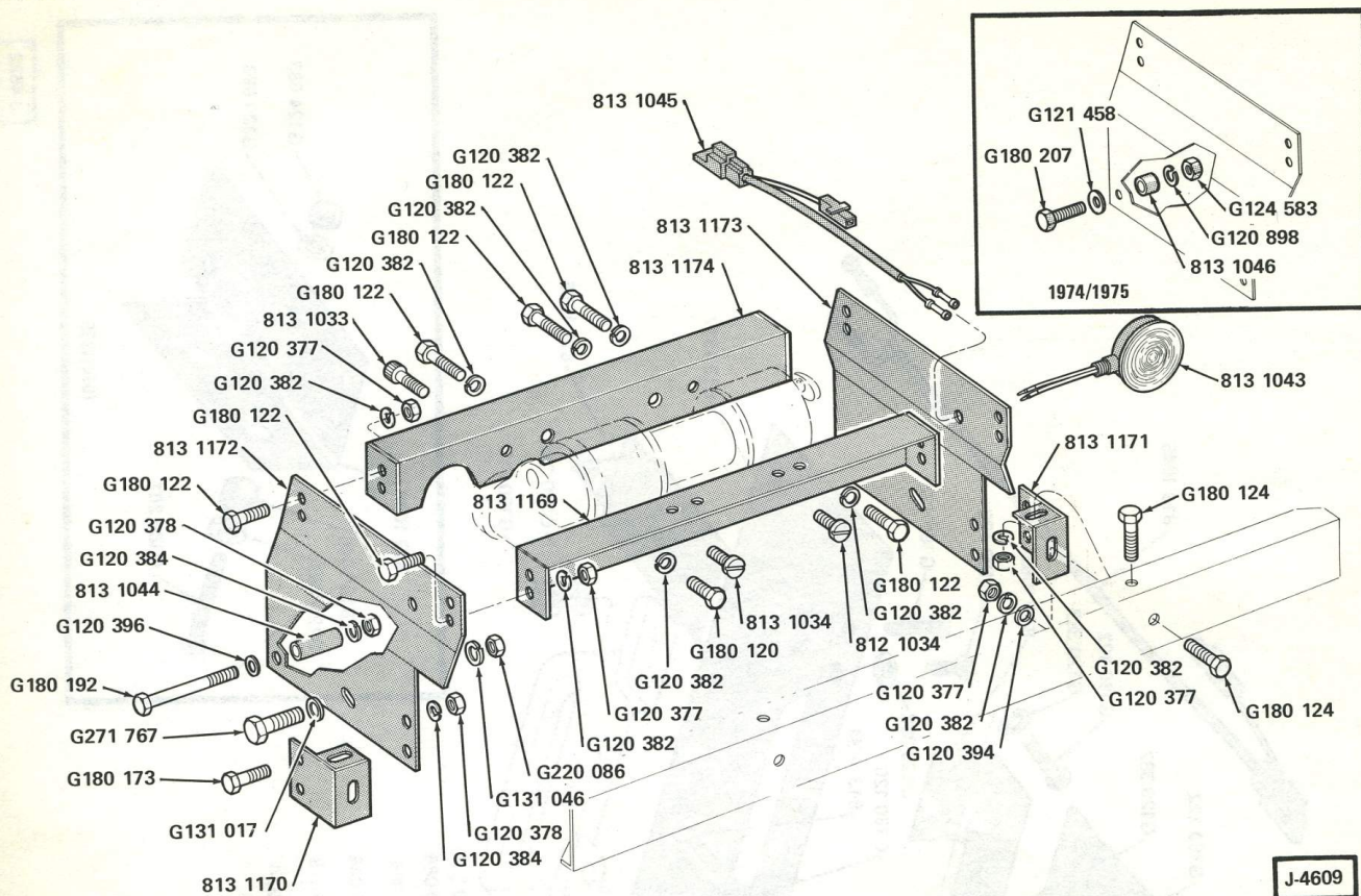
WINCH MOUNTING (RAMSEY) . . . 80-90 (LIGHTWEIGHT)
